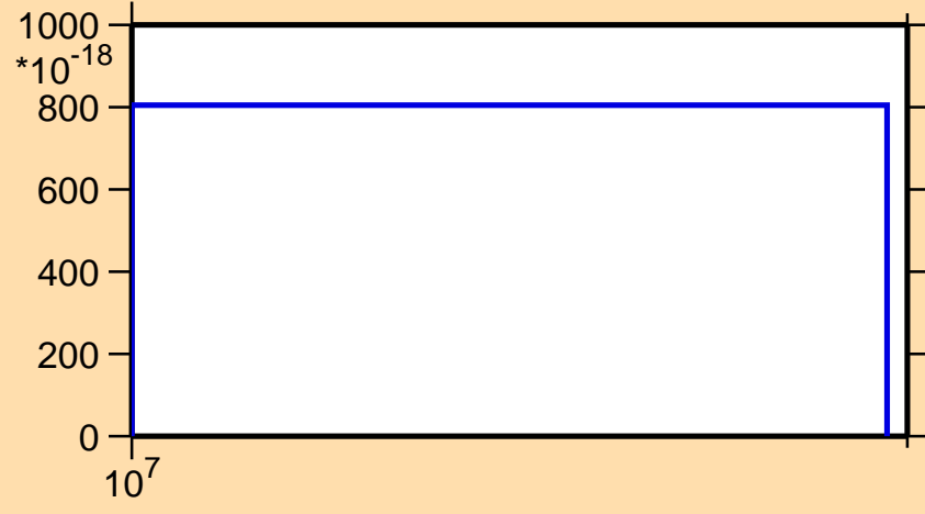
\sigma vs. E for ^{160}\text{Tm}(n,3n\alpha)
