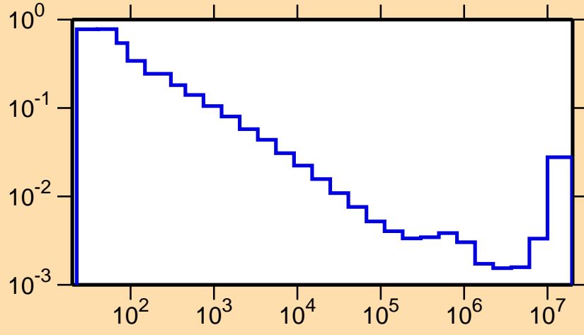
\sigma vs. E for ^{160}\text{Tm}(n,\alpha)
