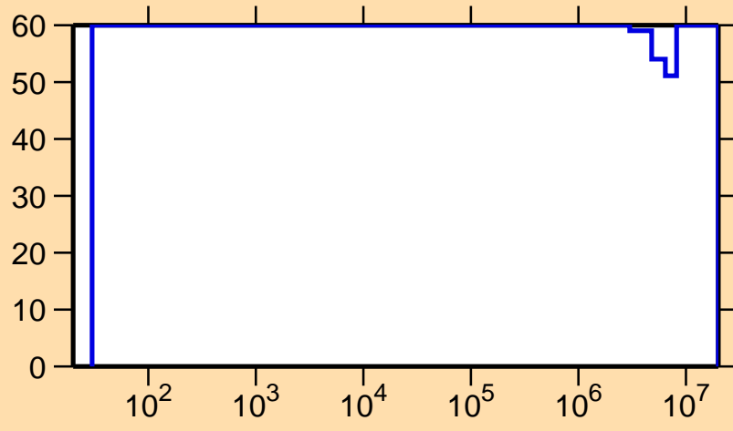
\Delta\sigma/\sigma vs. E for ^{160}\text{Tm}(n,p)
