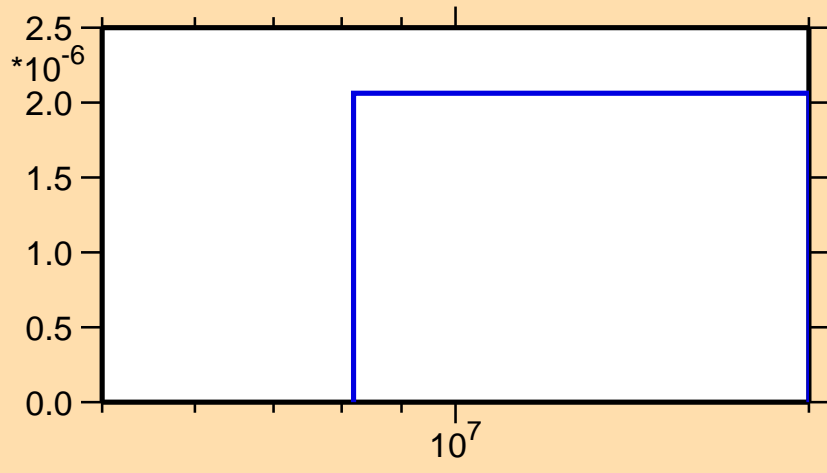
\sigma vs. E for ^{160}\text{Tm}(n,\text{nd})
