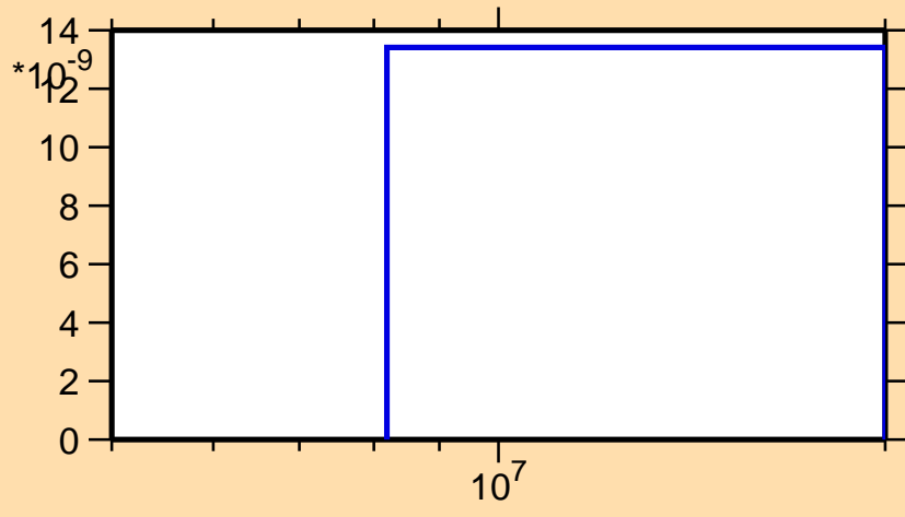
\sigma vs. E for ^{160}\text{Tm} (mt 45)
