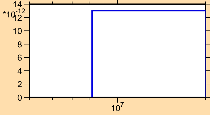
\sigma vs. E for ^{160}\text{Tm}(n,\text{pd})
