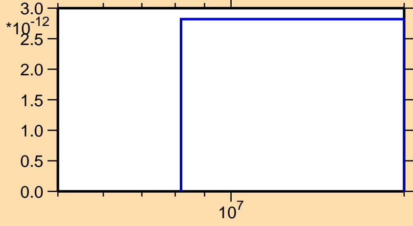
\sigma vs. E for ^{160}\text{Tm}(n,\text{pt})
