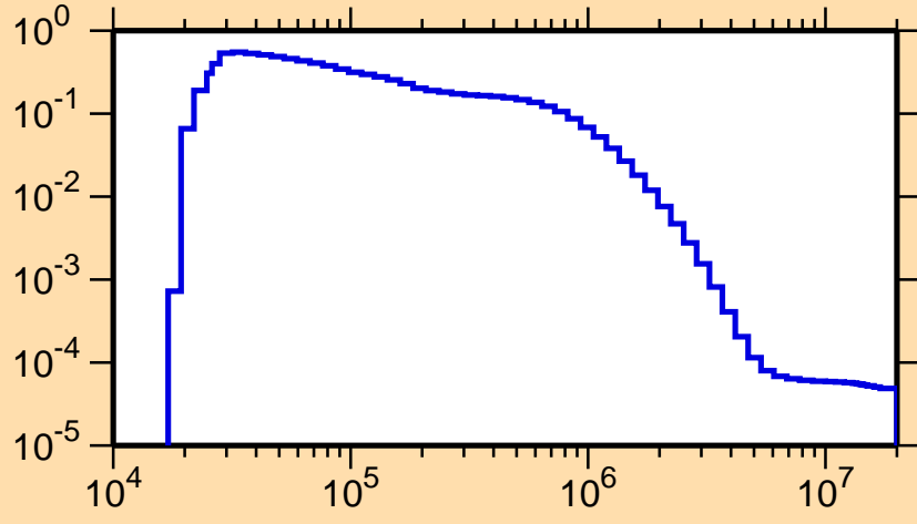
\sigma vs. E for ^{161}\text{Tm}(n,n_2)
