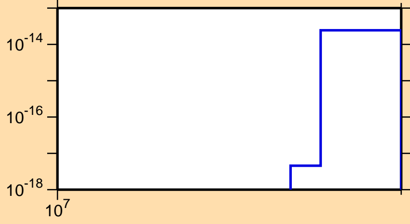
\sigma vs. E for ^{161}\text{Tm}(n,3n\alpha)
