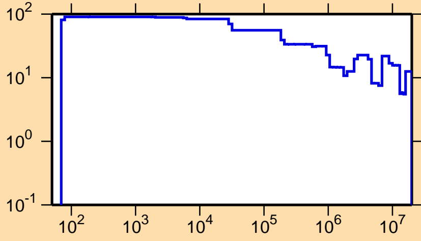
\Delta\sigma/\sigma vs. E for ^{161}\text{Tm}(n,el.)
