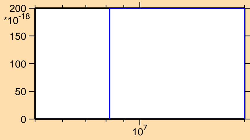
\sigma vs. E for ^{161}\text{Tm}(n,3n\alpha)
