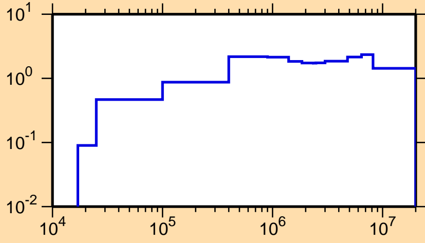
\sigma vs. E for ^{161}\text{Tm}(n,\text{inel.})
