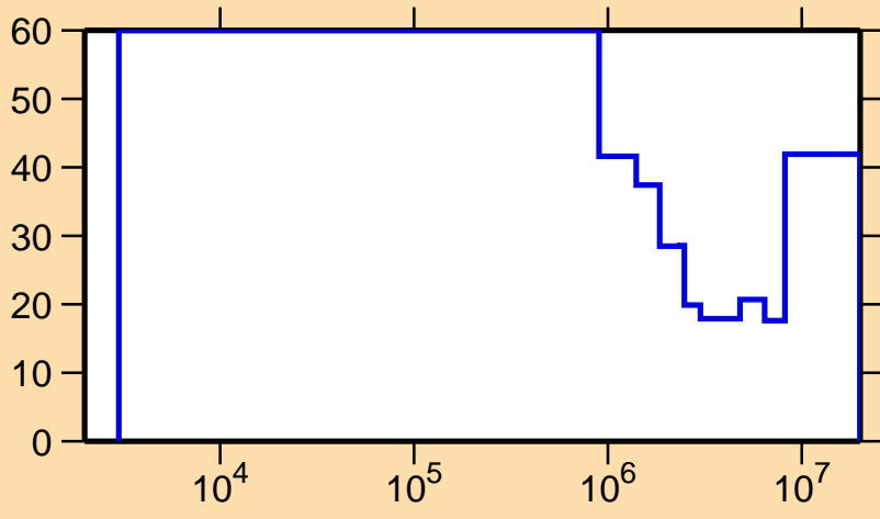
\Delta\sigma/\sigma vs. E for ^{161}\text{Tm}(n,\text{inel.})
