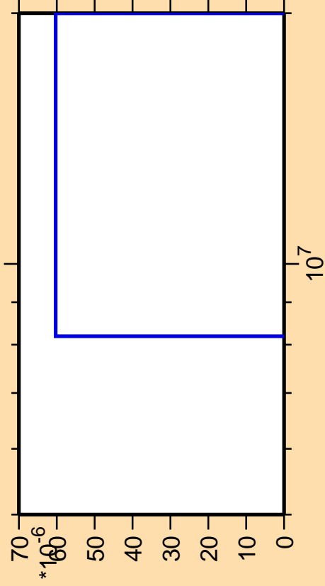
\Delta\sigma/\sigma vs. E for ^{161}\text{Tm}(n,3n\alpha)
