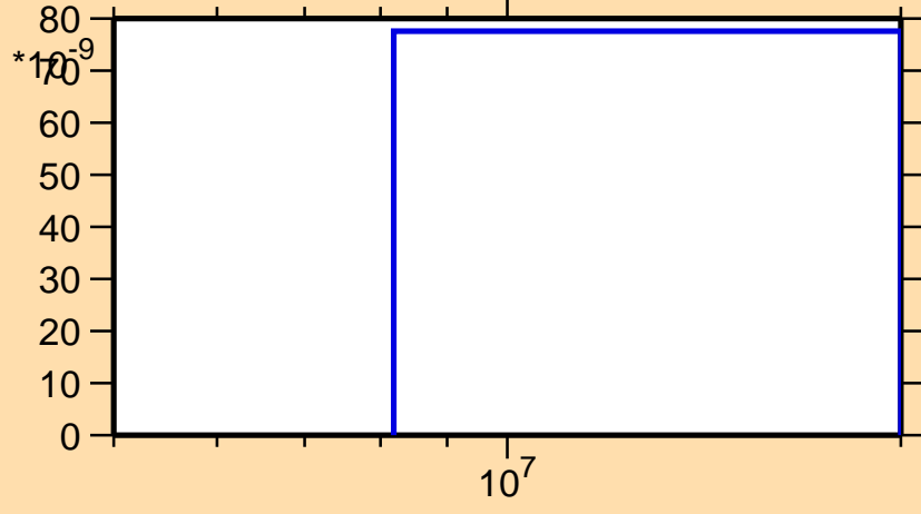
\sigma vs. E for ^{161}\text{Tm}(n,nd)
