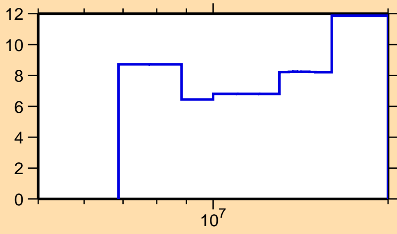
\Delta\sigma/\sigma vs. E for ^{162}\text{Tm}(n,\text{tot.})
