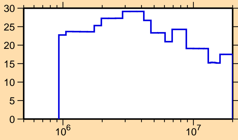
\Delta\sigma/\sigma vs. E for ^{162}\text{Tm}(n, el.)
