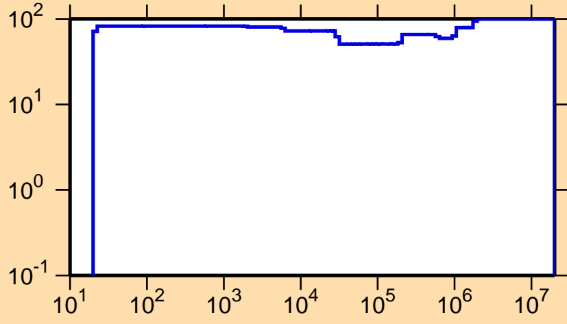
\Delta\sigma/\sigma vs. E for ^{162}\text{Tm}(n,\gamma)
