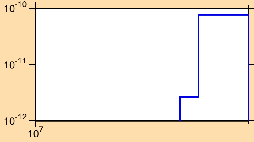
\sigma vs. E for ^{162}\text{Tm}(n,\text{pd})
