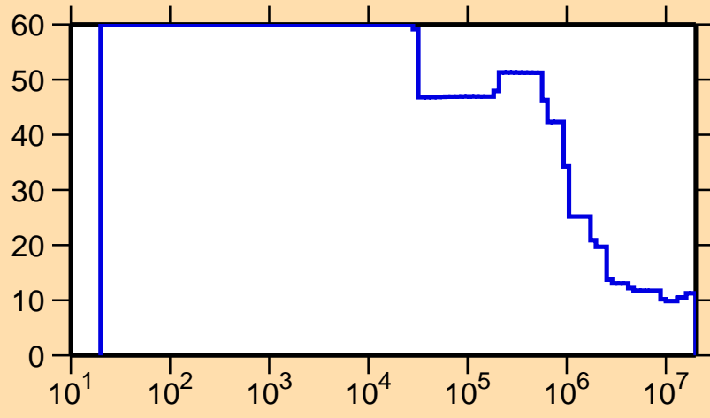
\Delta\sigma/\sigma vs. E for ^{162}\text{Tm}(n,\text{nonel.})
