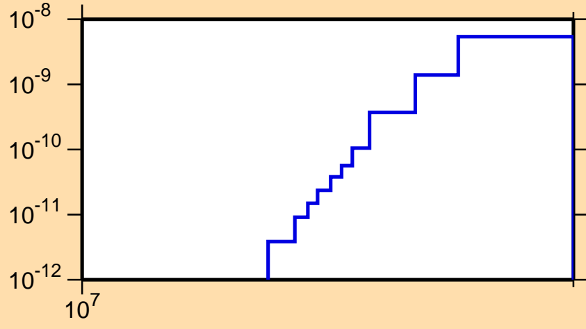
\sigma vs. E for ^{162}\text{Tm}(\text{mt117})
