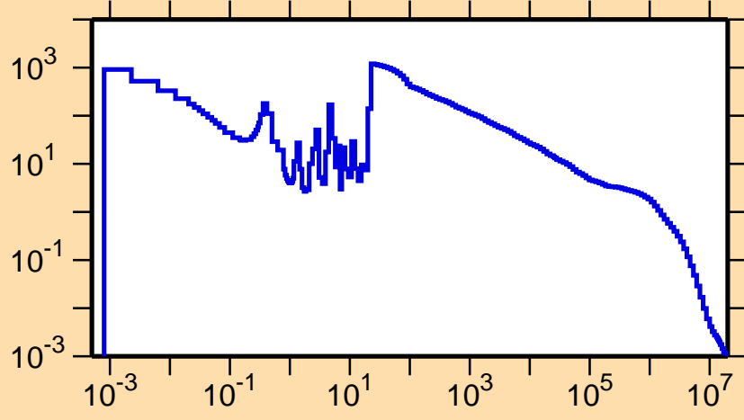
\sigma vs. E for ^{162}\text{Tm}(n,\gamma)
