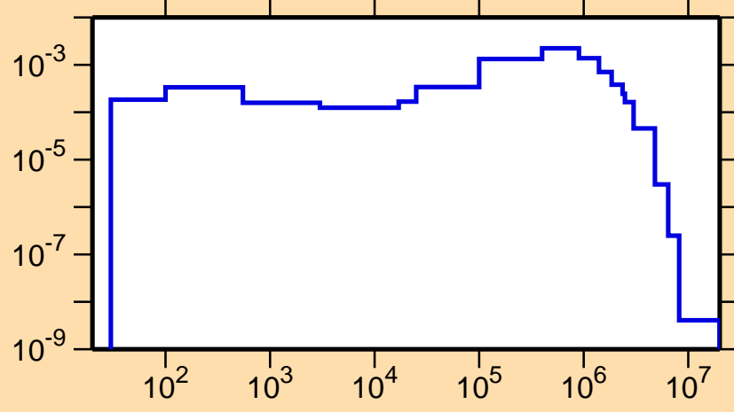
\sigma vs. E for ^{162}\text{Tm}(n,n_3)
