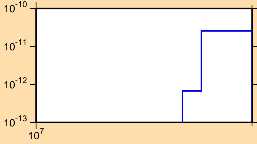
\sigma vs. E for ^{163}\text{Tm}(n,\text{pd})
