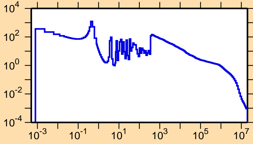
\sigma vs. E for ^{163}\text{Tm}(n,\gamma)
