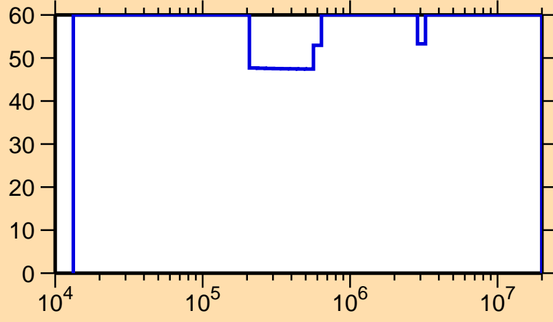
\Delta\sigma/\sigma vs. E for ^{163}\text{Tm}(n,n_1)
