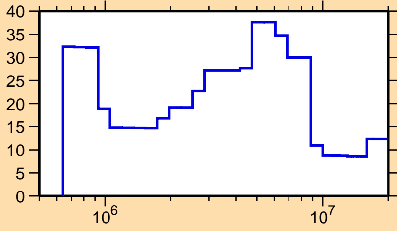
\Delta\sigma/\sigma vs. E for ^{163}\text{Tm}(n,el.)
