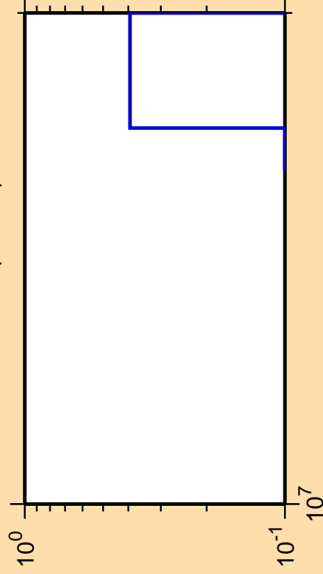
\Delta\sigma/\sigma vs. E for ^{163}\text{Tm} (mt 34)
