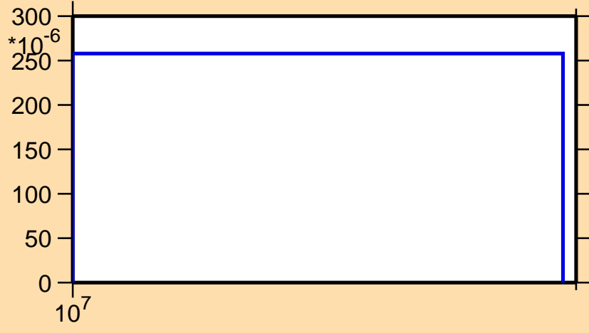
\sigma vs. E for ^{163}\text{Tm}(n,3n)
