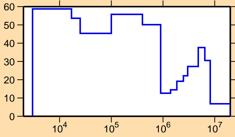
\Delta\sigma/\sigma vs. E for ^{163}\text{Tm}(n,\text{el.})
