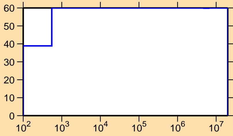
\Delta\sigma/\sigma vs. E for ^{163}\text{Tm}(n,p)
