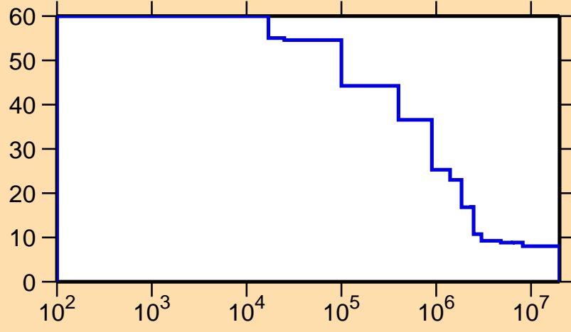
\Delta\sigma/\sigma vs. E for ^{163}\text{Tm}(n,\text{nonel.})
