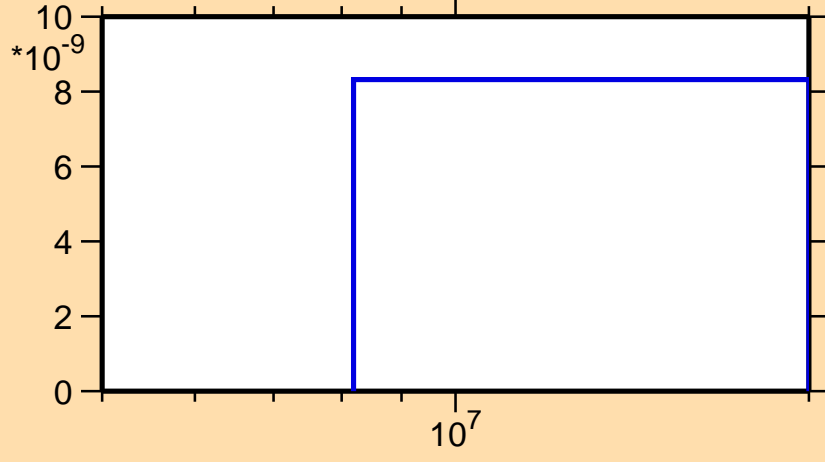
\sigma vs. E for ^{163}\text{Tm}(n,\text{He}3)
