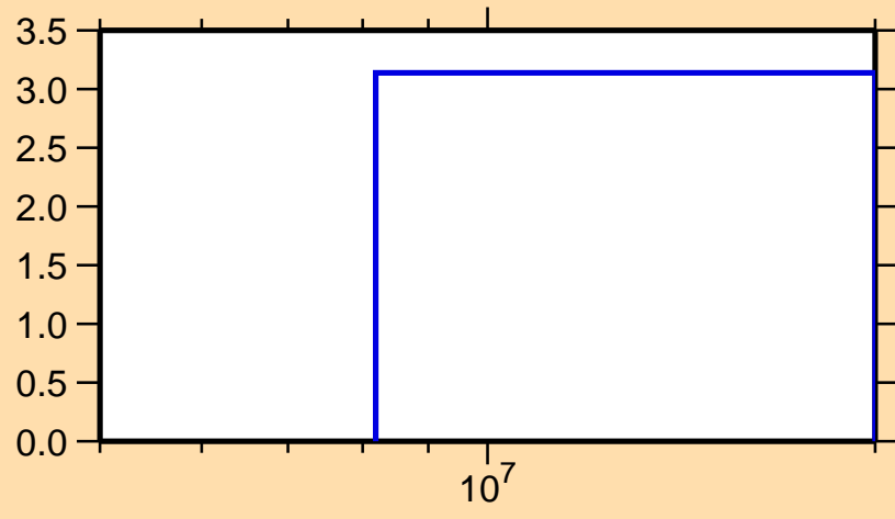
\Delta\sigma/\sigma vs. E for ^{163}\text{Tm}(n,\text{tot.})
