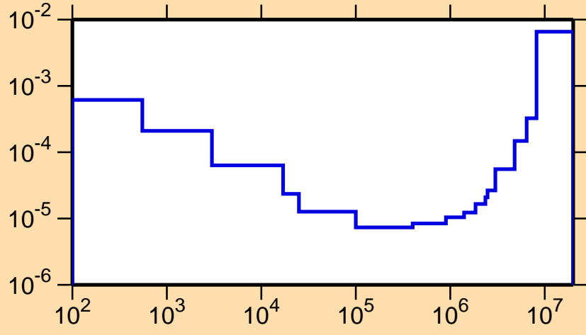
\sigma vs. E for ^{163}\text{Tm}(n,\alpha)
