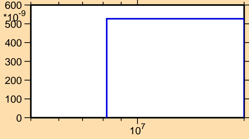
\sigma vs. E for ^{163}\text{Tm}(n,2np)
