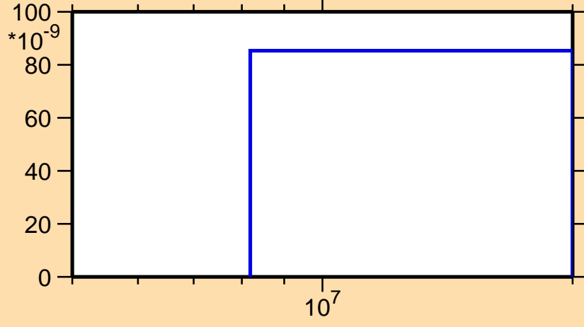
\sigma vs. E for ^{163}\text{Tm}(n,2n\alpha)
