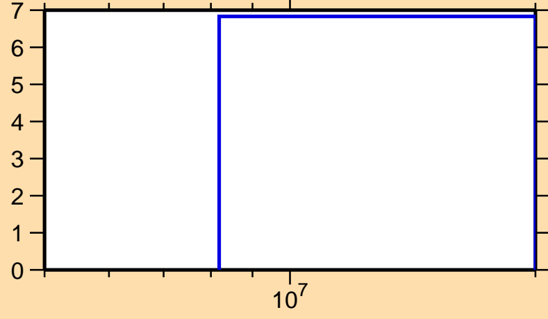
\Delta\sigma/\sigma vs. E for ^{163}\text{Tm}(n,\text{el.})
