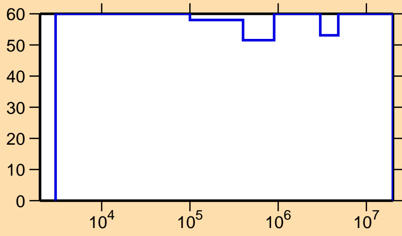
\Delta\sigma/\sigma vs. E for ^{163}\text{Tm}(n,n_1)
