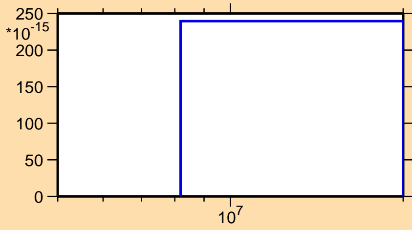
\sigma vs. E for ^{163}\text{Tm}(n,\text{pd})
