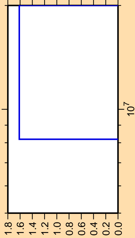
\Delta\sigma/\sigma vs. E for ^{163}\text{Tm}(n,\text{pd})
