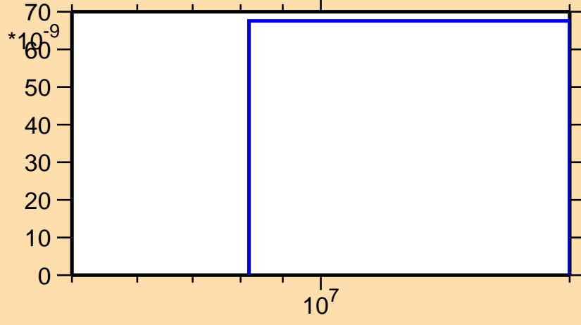
\sigma vs. E for ^{163}\text{Tm}(n,nd)
