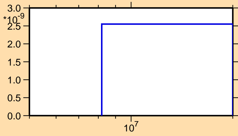
\sigma vs. E for ^{163}\text{Tm}(n,nt)
