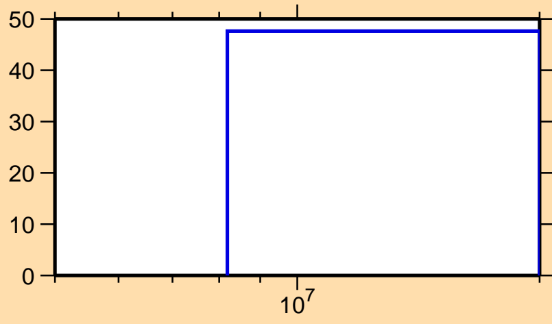
\Delta\sigma/\sigma vs. E for ^{163}\text{Tm}(n,\text{inel.})
