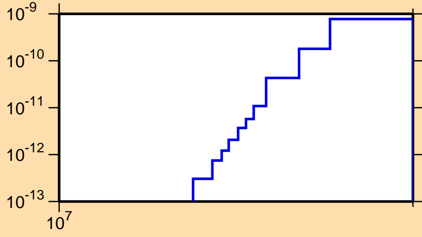
\sigma vs. E for ^{164}\text{Tm}(\text{mt117})
