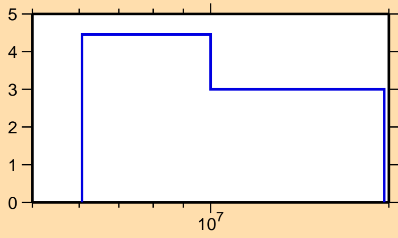
\Delta\sigma/\sigma vs. E for ^{164}\text{Tm}(n,\text{nonel.})
