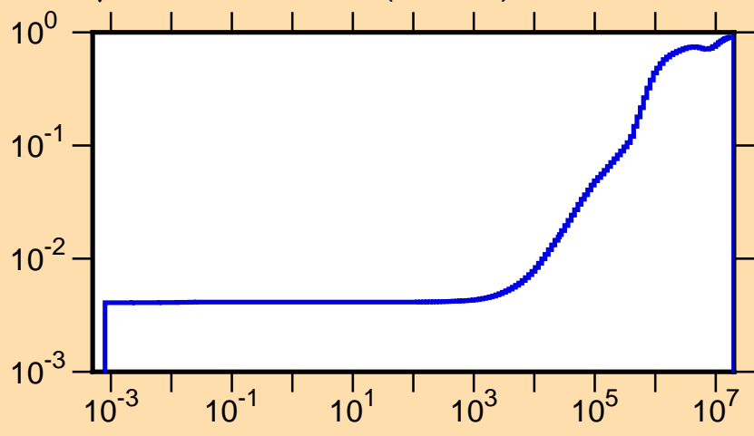
\mu vs. E for ^{165}\text{Tm}(\text{mt251})
