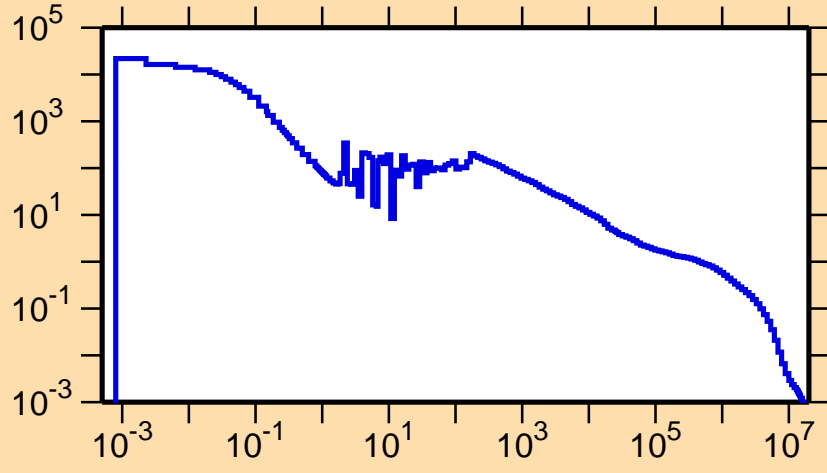
\sigma vs. E for ^{165}\text{Tm}(n,\gamma)
