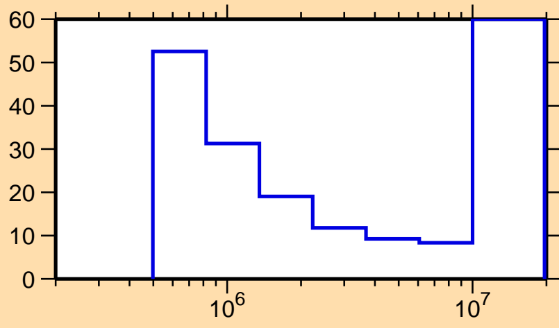
\Delta\sigma/\sigma vs. E for ^{165}\text{Tm}(n,n\text{cont.})
