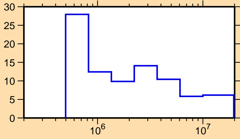
\Delta\sigma/\sigma vs. E for ^{165}\text{Tm}(n,nonel.)
