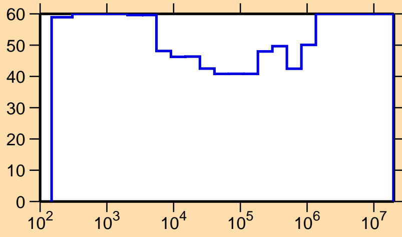
\Delta\sigma/\sigma vs. E for ^{165}\text{Tm}(n,\gamma)
