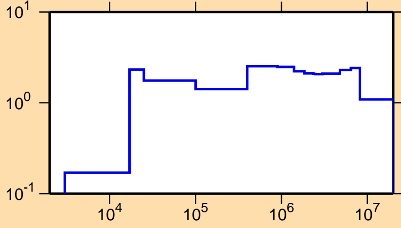
\sigma vs. E for ^{165}\text{Tm}(n,\text{inel.})
