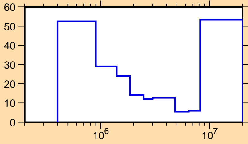
\Delta\sigma/\sigma vs. E for ^{165}\text{Tm}(n,ncont.)
