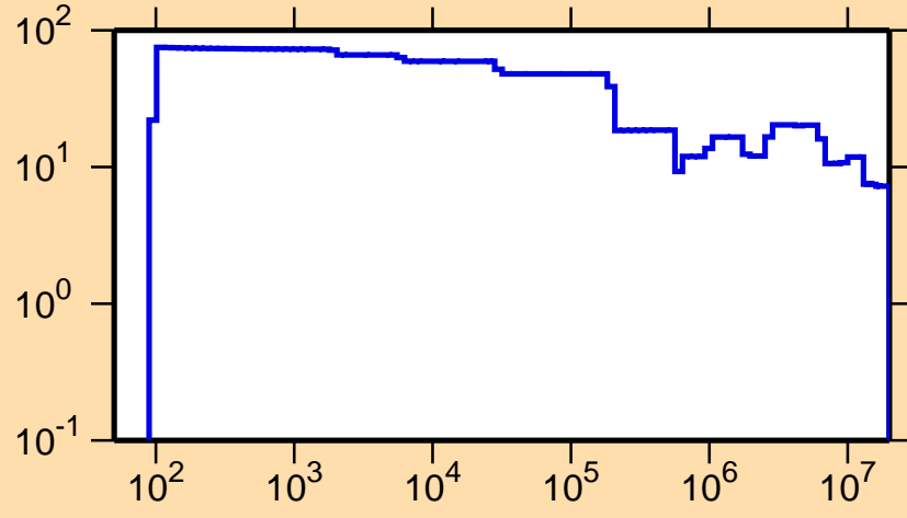
\Delta\sigma/\sigma vs. E for ^{166}\text{Tm}(n,el.)
