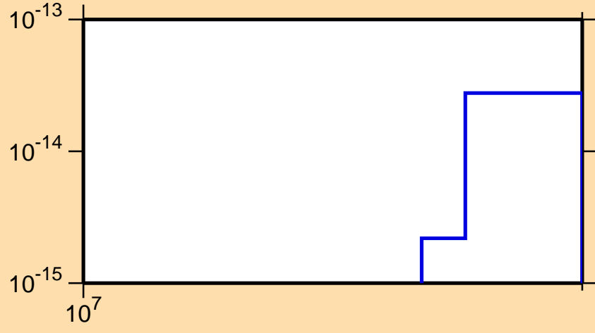
\sigma vs. E for ^{166}\text{Tm}(n,3n\alpha)
