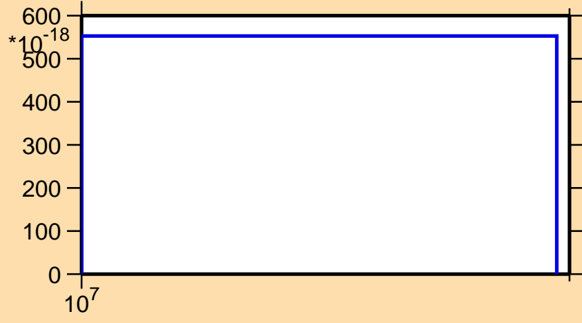
\sigma vs. E for ^{166}\text{Tm}(n,3n\alpha)
