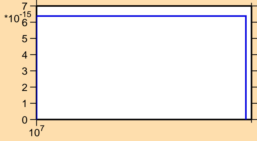
\sigma vs. E for ^{166}\text{Tm} (mt 34)
