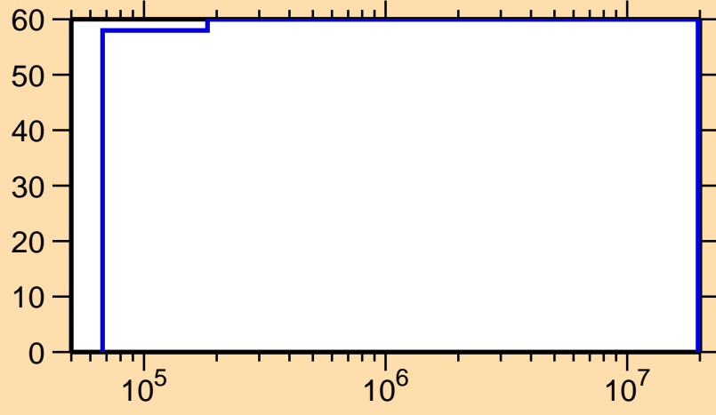
\Delta\sigma/\sigma vs. E for ^{166}\text{Tm}(n,n_1)
