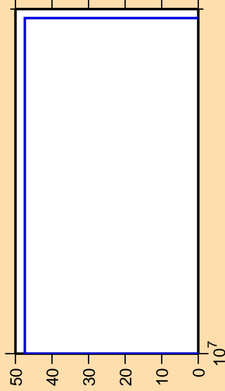
\Delta\sigma/\sigma vs. E for ^{166}\text{Tm}(n,3n)
