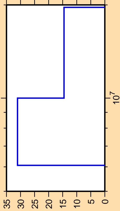
\Delta\sigma/\sigma vs. E for ^{166}\text{Tm}(n,2n)
