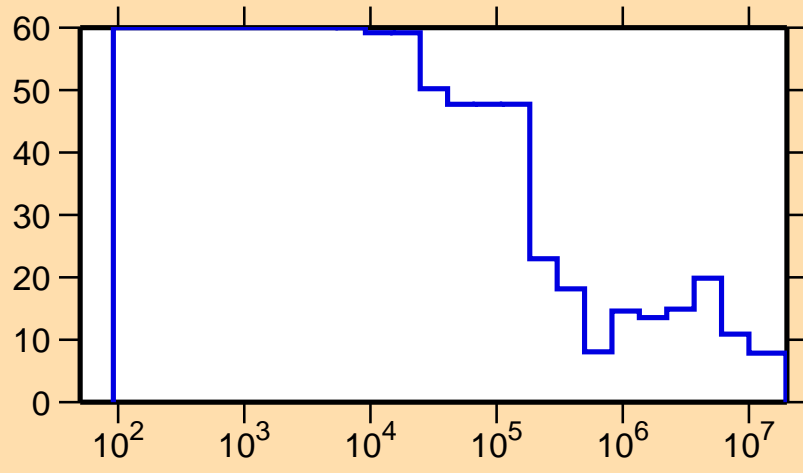
\Delta\sigma/\sigma vs. E for ^{166}\text{Tm}(n,el.)
