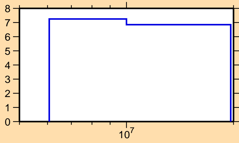
\Delta\sigma/\sigma vs. E for ^{166}\text{Tm}(n,\text{nonel.})
