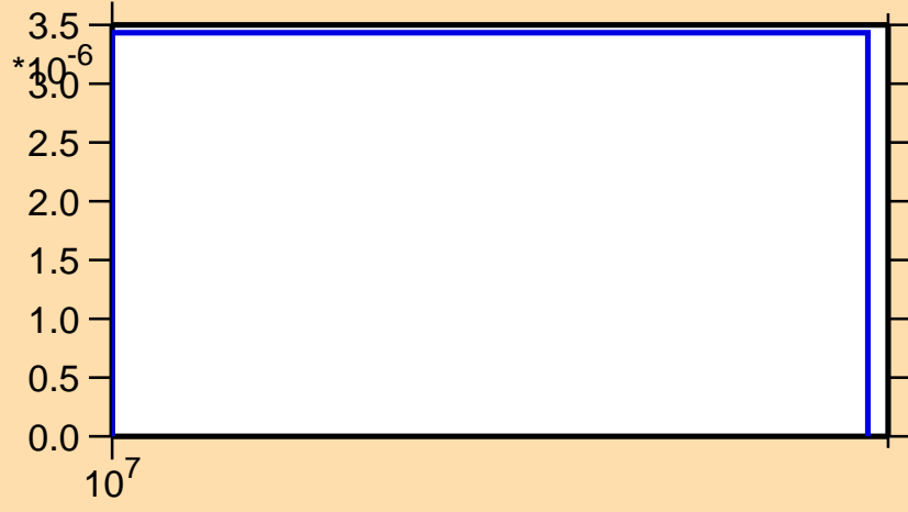
\sigma vs. E for ^{166}\text{Tm}(n,2np)
