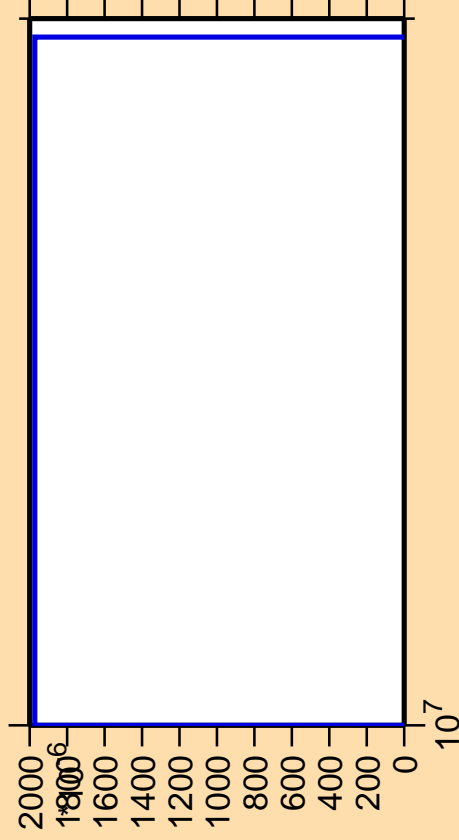
\Delta\sigma/\sigma vs. E for ^{166}\text{Tm}(n,3n\alpha)
