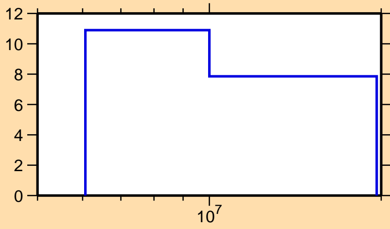
\Delta\sigma/\sigma vs. E for ^{166}\text{Tm}(n,\text{el.})
