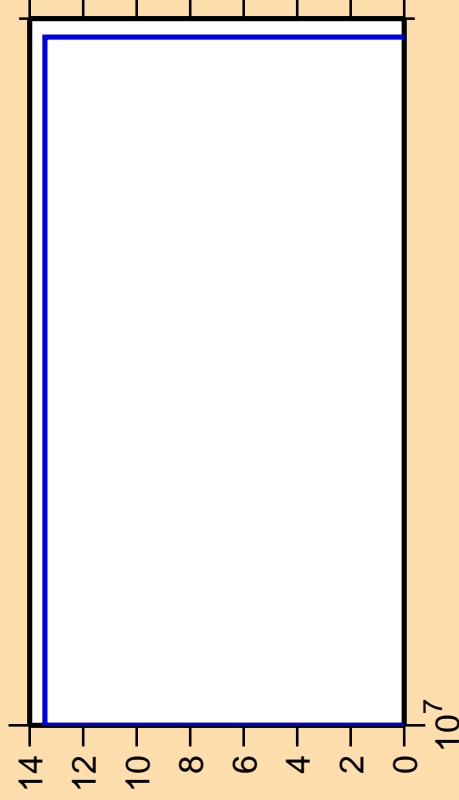
\Delta\sigma/\sigma vs. E for ^{166}\text{Tm}(\text{mt117})
