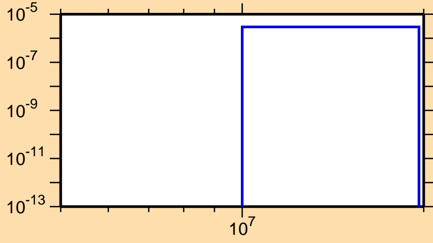
\sigma vs. E for ^{166}\text{Tm}(n,2n\alpha)
