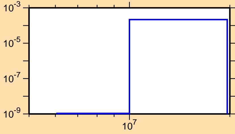
\sigma vs. E for ^{166}\text{Tm}(n,t)
