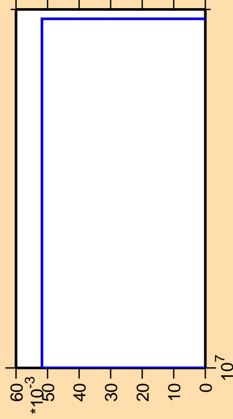
\Delta\sigma/\sigma vs. E for ^{166}\text{Tm} (mt 34)
