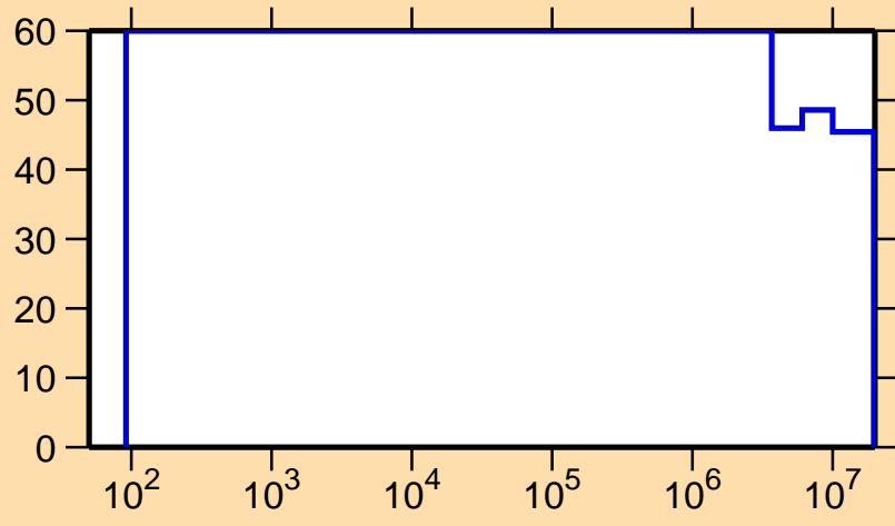
\Delta\sigma/\sigma vs. E for ^{166}\text{Tm}(n,p)
