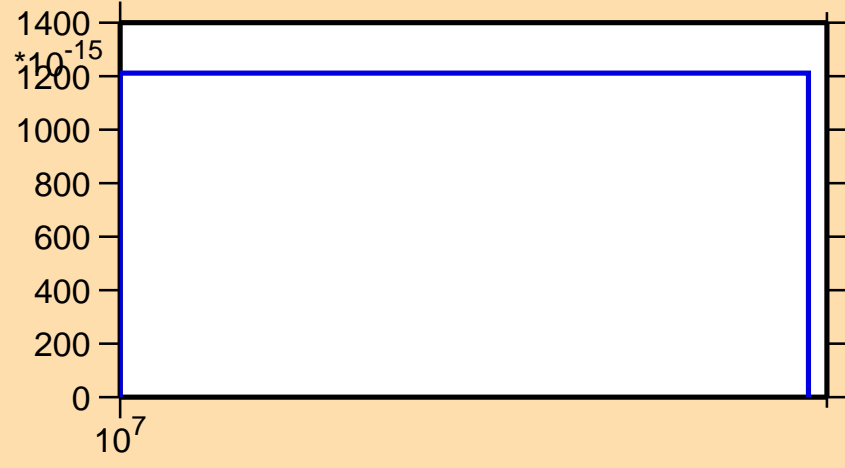
\sigma vs. E for ^{166}\text{Tm} (mt 45)
