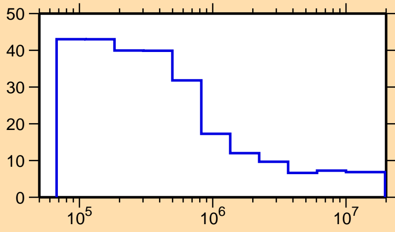
\Delta\sigma/\sigma vs. E for ^{166}\text{Tm}(n,\text{nonel.})
