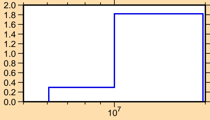
\sigma vs. E for ^{166}\text{Tm}(n,2n)
