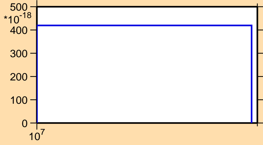
\sigma vs. E for ^{166}\text{Tm}(n,\text{pd})
