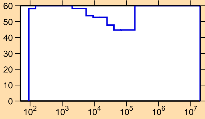
\Delta\sigma/\sigma vs. E for ^{166}\text{Tm}(n,\gamma)
