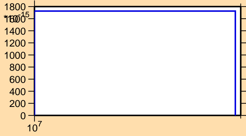
\sigma vs. E for ^{166}\text{Tm}(\text{mt117})
