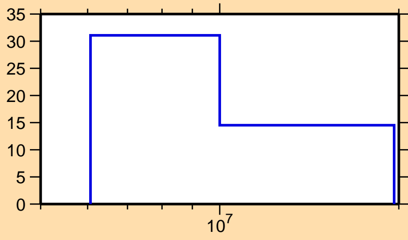
\Delta\sigma/\sigma vs. E for ^{166}\text{Tm}(n,2n)
