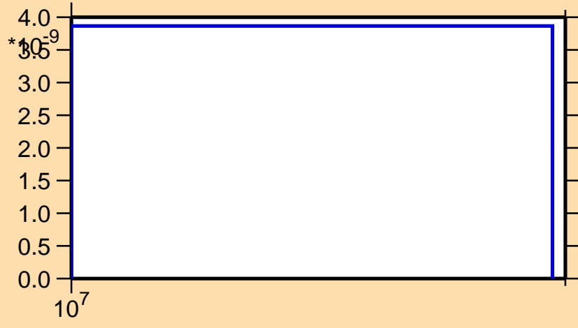
\sigma vs. E for ^{166}\text{Tm}(n,\text{He}3)
