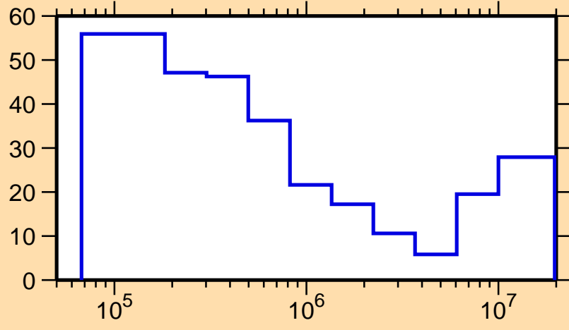
\Delta\sigma/\sigma vs. E for ^{166}\text{Tm}(n,\text{inel.})
