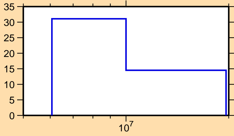
\Delta\sigma/\sigma vs. E for ^{166}\text{Tm}(n,2n)
