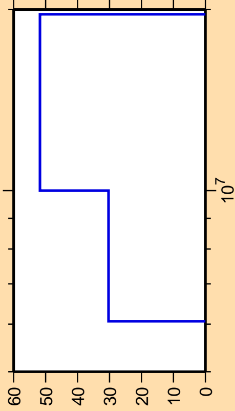
\Delta\sigma/\sigma vs. E for ^{166}\text{Tm}(n,n\text{cont.})
