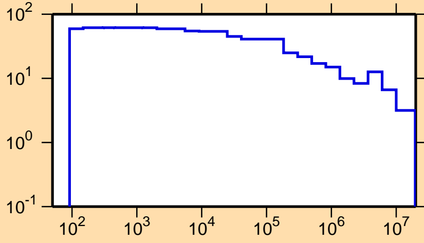
\Delta\sigma/\sigma vs. E for ^{166}\text{Tm}(n,\text{tot.})
