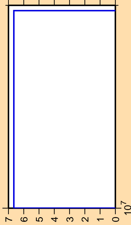
\Delta\sigma/\sigma vs. E for ^{166}\text{Tm} (mt 45)
