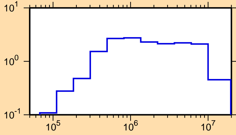
\sigma vs. E for ^{166}\text{Tm}(n,\text{inel.})
