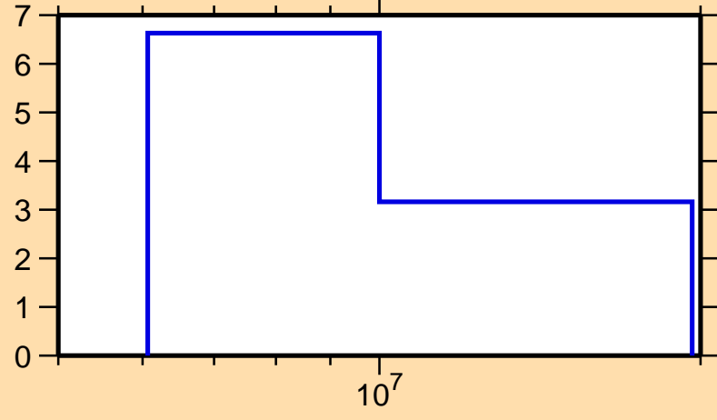
\Delta\sigma/\sigma vs. E for ^{166}\text{Tm}(n,\text{tot.})
