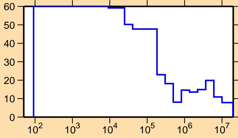
\Delta\sigma/\sigma vs. E for ^{166}\text{Tm}(n,\text{el.})
