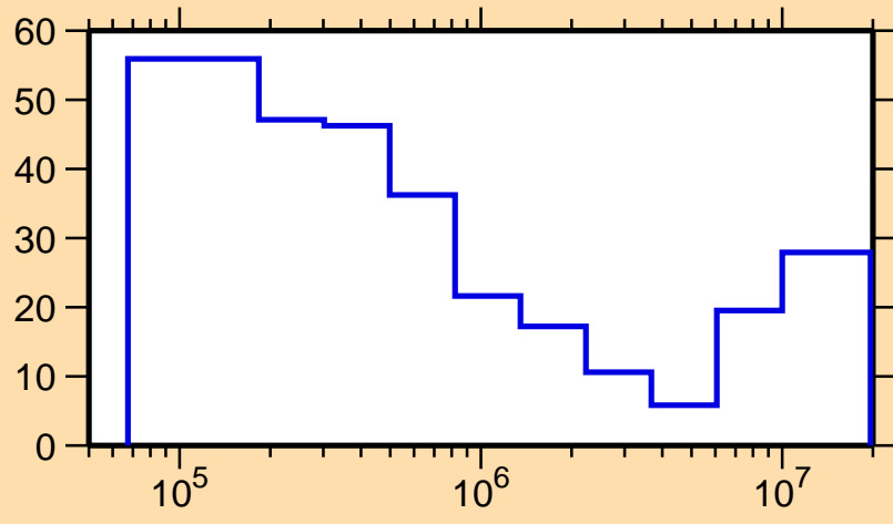
\Delta\sigma/\sigma vs. E for ^{166}\text{Tm}(n,\text{inel.})
