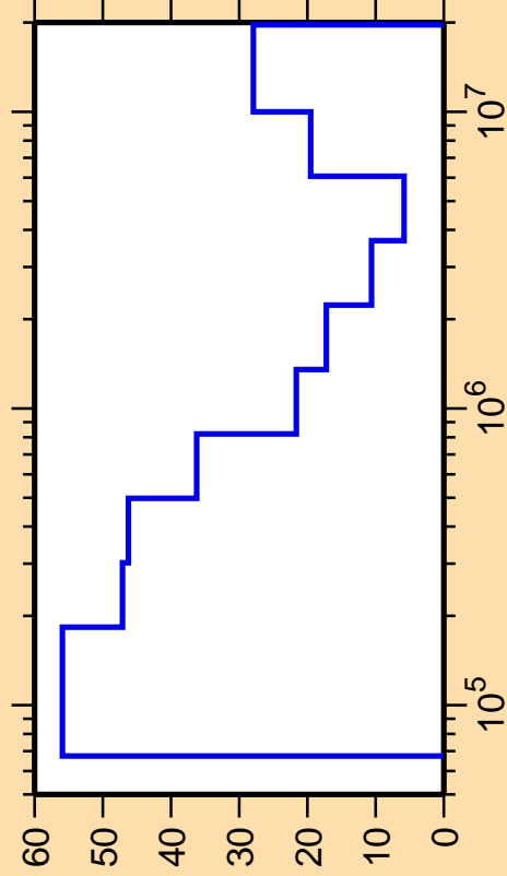
\Delta\sigma/\sigma vs. E for ^{166}\text{Tm}(n,\text{inel.})
