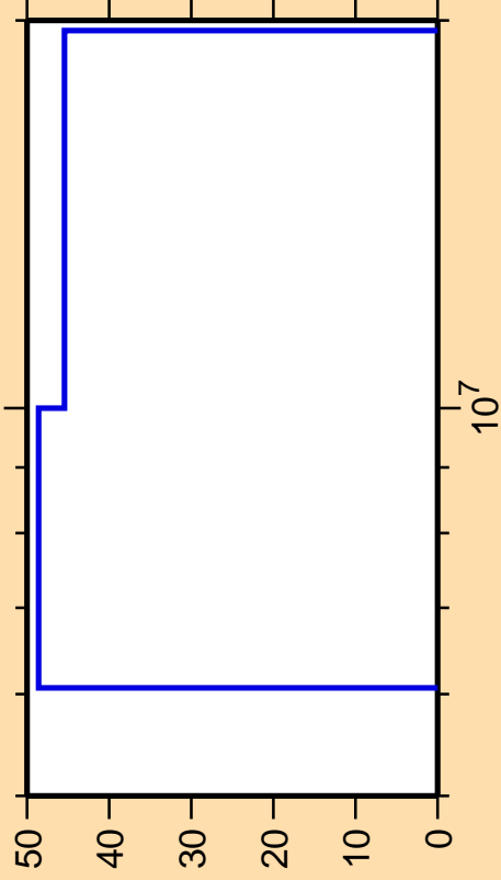
\Delta\sigma/\sigma vs. E for ^{166}\text{Tm}(n,p)
