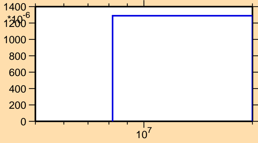
\sigma vs. E for ^{166}\text{Tm}(n,3n)
