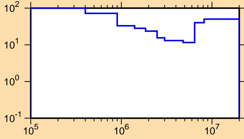
\Delta\sigma/\sigma vs. E for ^{166}\text{Tm}(n,n\text{cont.})
