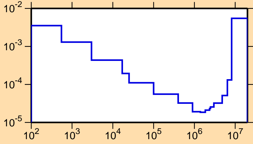
\sigma vs. E for ^{166}\text{Tm}(n,\alpha)
