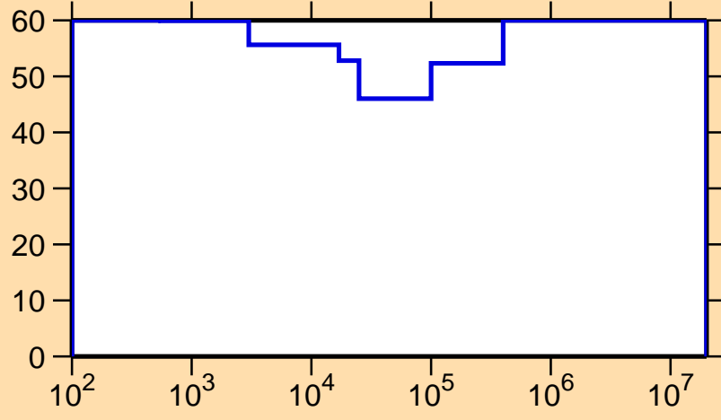
\Delta\sigma/\sigma vs. E for ^{166}\text{Tm}(n,\gamma)
