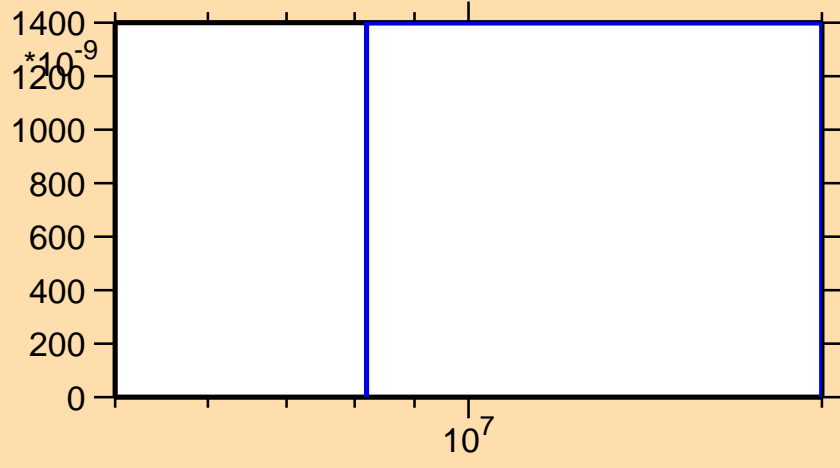
\sigma vs. E for ^{166}\text{Tm}(n,\text{nd})
