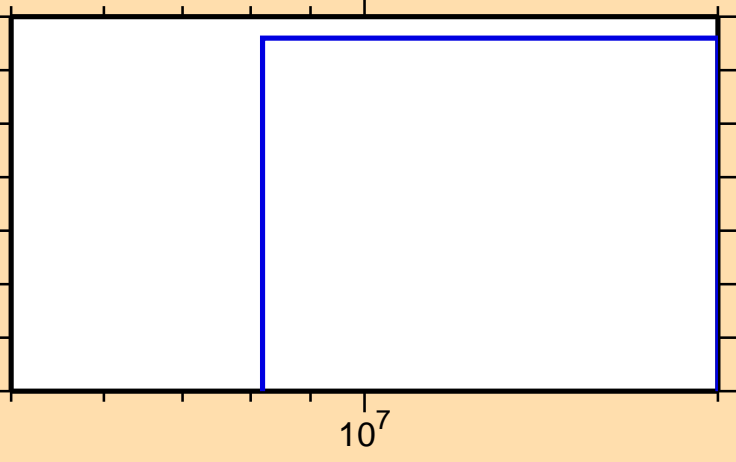
\sigma vs. E for ^{166}\text{Tm}(n,nt)
