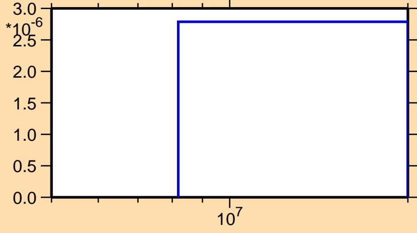
\sigma vs. E for ^{166}\text{Tm}(n,2np)
