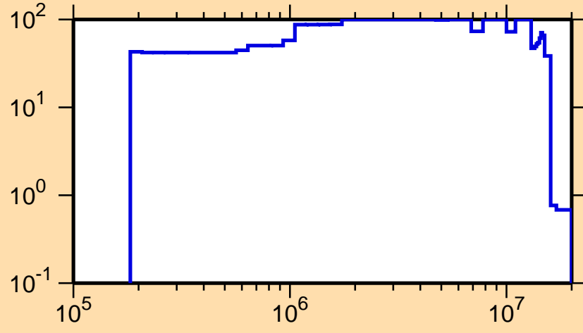
\Delta\sigma/\sigma vs. E for ^{167}\text{Tm}(n,n_1)
