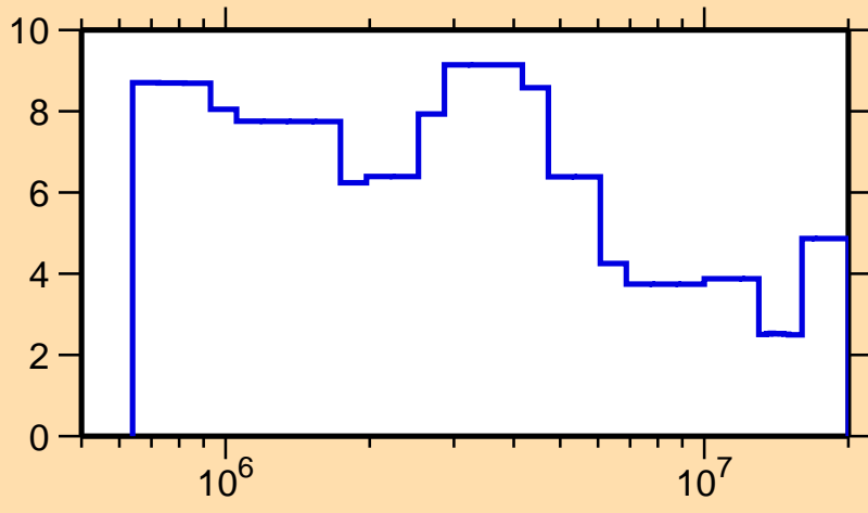
\Delta\sigma/\sigma vs. E for ^{167}\text{Tm}(n,\text{tot.})
