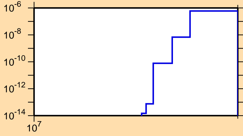
\sigma vs. E for ^{167}\text{Tm}(n,nt)
