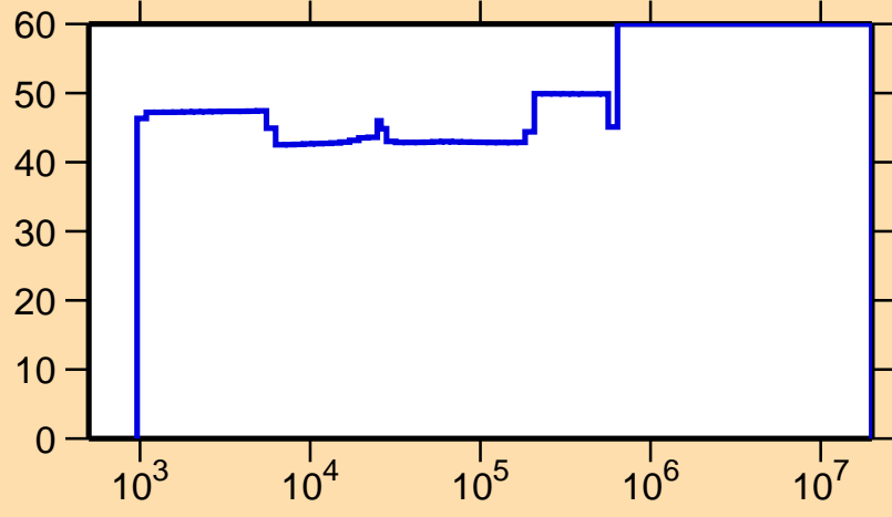
\Delta\sigma/\sigma vs. E for ^{167}\text{Tm}(n,\gamma)
