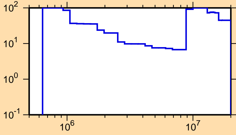
\Delta\sigma/\sigma vs. E for ^{167}\text{Tm}(n,n\text{cont.})
