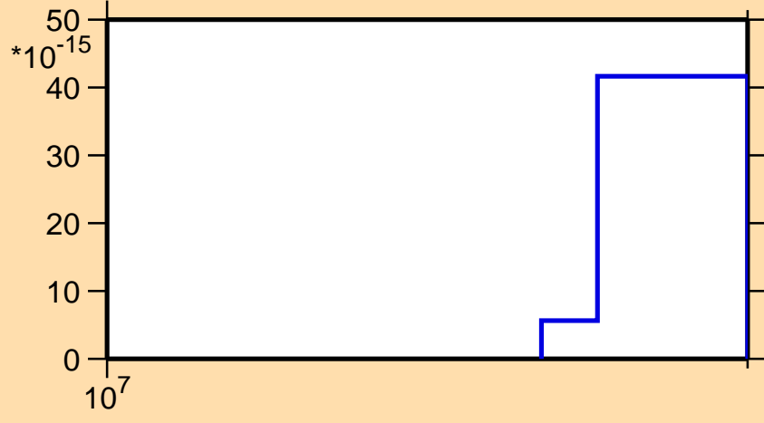
\sigma vs. E for ^{167}\text{Tm}(n,3n\alpha)
