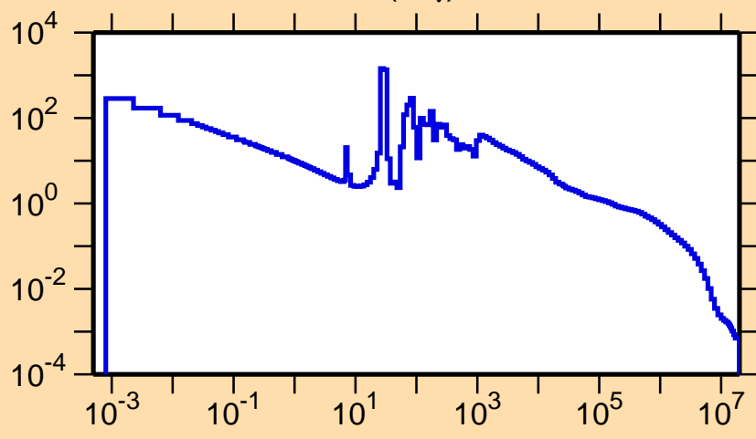
\sigma vs. E for ^{167}\text{Tm}(n,\gamma)
