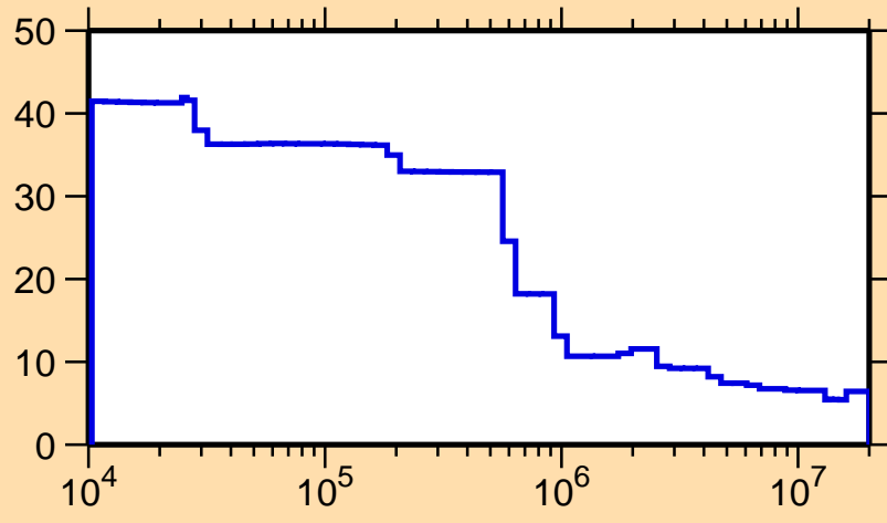
\Delta\sigma/\sigma vs. E for ^{167}\text{Tm}(n,\text{nonel.})
