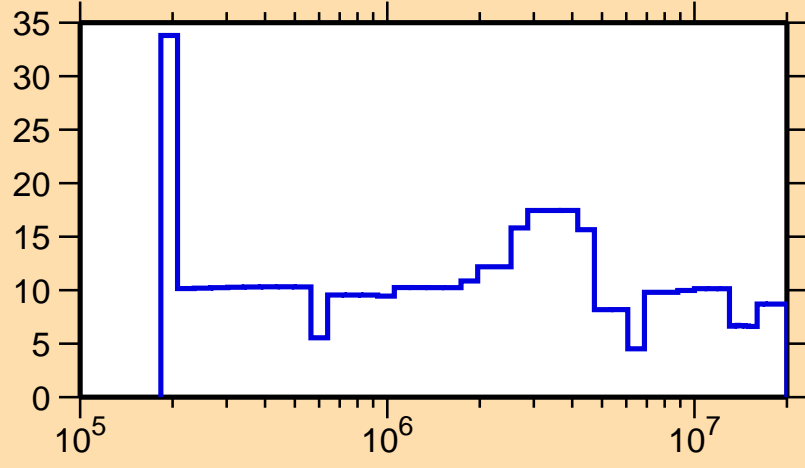
\Delta\sigma/\sigma vs. E for ^{167}\text{Tm}(n,el.)
