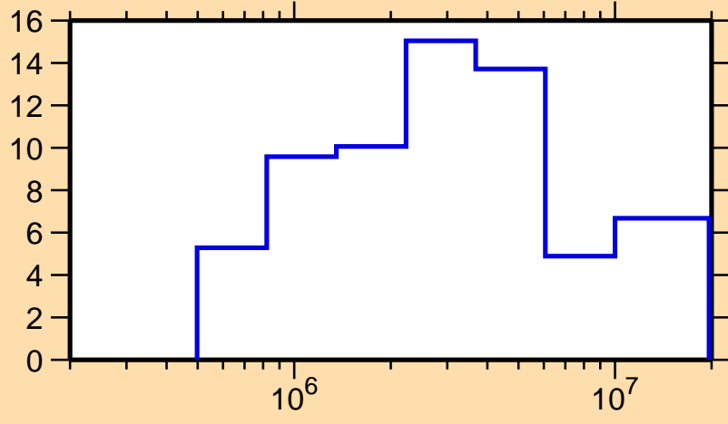
\Delta\sigma/\sigma vs. E for ^{167}\text{Tm}(n, el.)
