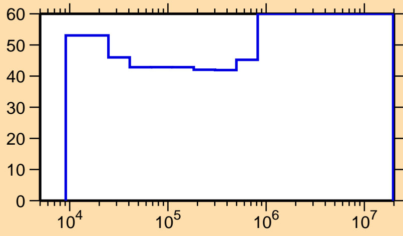
\Delta\sigma/\sigma vs. E for ^{167}\text{Tm}(n,n_1)
