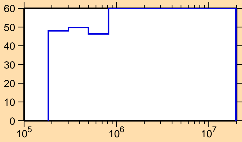
\Delta\sigma/\sigma vs. E for ^{167}\text{Tm}(n,\gamma)
