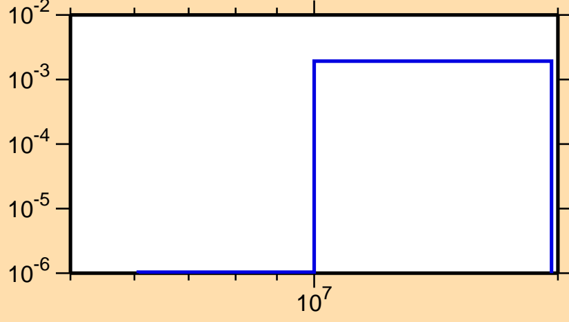
\sigma vs. E for ^{167}\text{Tm}(n,np)
