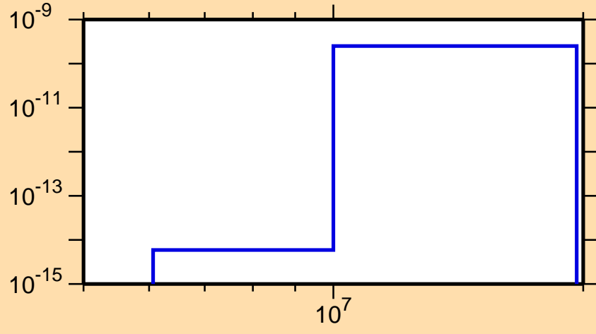
\sigma vs. E for ^{167}\text{Tm}(n,p\alpha)
