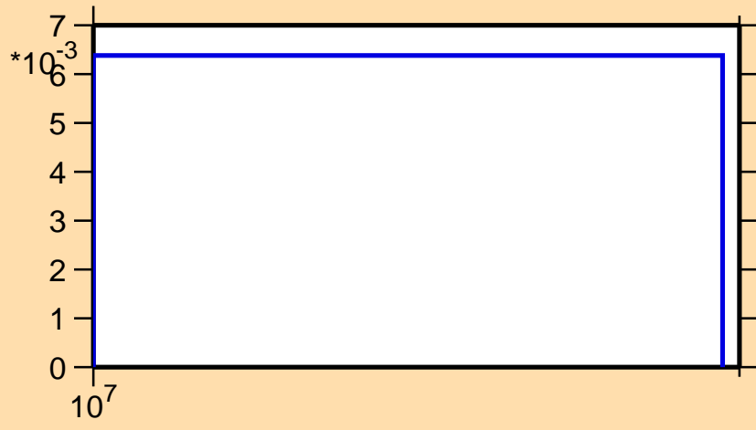
\sigma vs. E for ^{167}\text{Tm}(n,3n)
