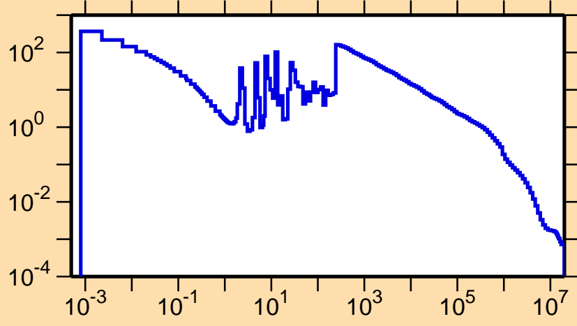
\sigma vs. E for ^{168}\text{Tm}(n,\gamma)
