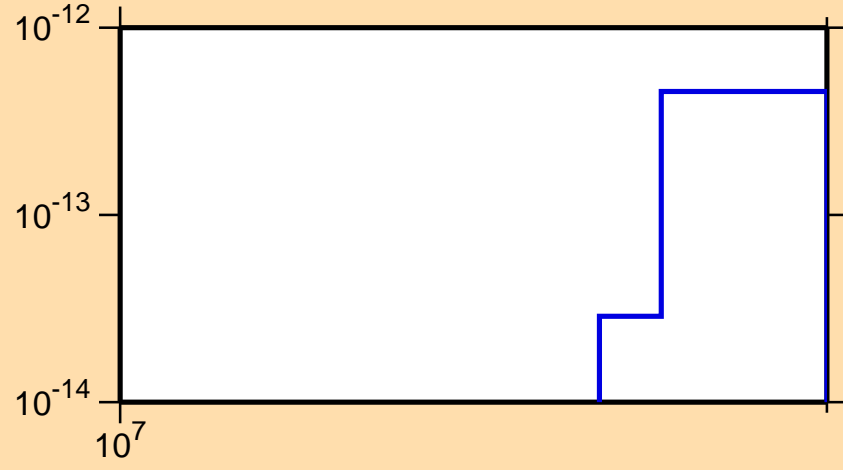
\sigma vs. E for ^{168}\text{Tm} (mt 45)
