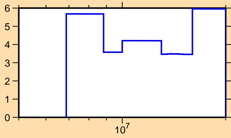
\Delta\sigma/\sigma vs. E for ^{168}\text{Tm}(n,\text{el.})
