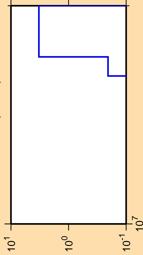
\Delta\sigma/\sigma vs. E for ^{168}\text{Tm} (mt 45)
