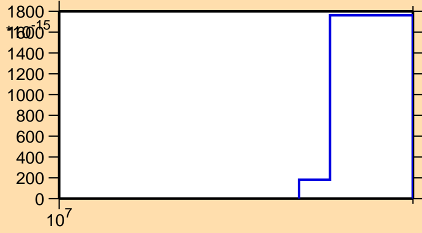
\sigma vs. E for ^{168}\text{Tm}(\text{mt117})
