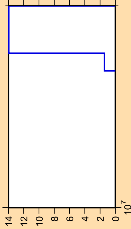
\Delta\sigma/\sigma vs. E for ^{168}\text{Tm}(\text{mt117})
