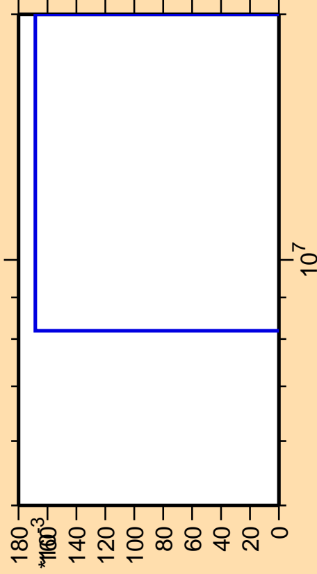
\Delta\sigma/\sigma vs. E for ^{168}\text{Tm}(\text{mt117})
