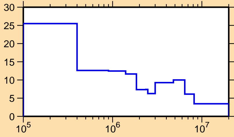
\Delta\sigma/\sigma vs. E for ^{168}\text{Tm}(n, tot.)
