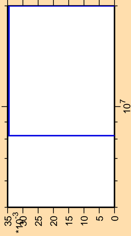
\Delta\sigma/\sigma vs. E for ^{168}\text{Tm} (mt 45)
