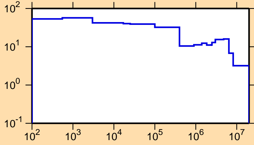
\Delta\sigma/\sigma vs. E for ^{168}\text{Tm}(n,el.)
