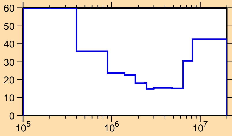
\Delta\sigma/\sigma vs. E for ^{168}\text{Tm}(n,n\text{cont.})
