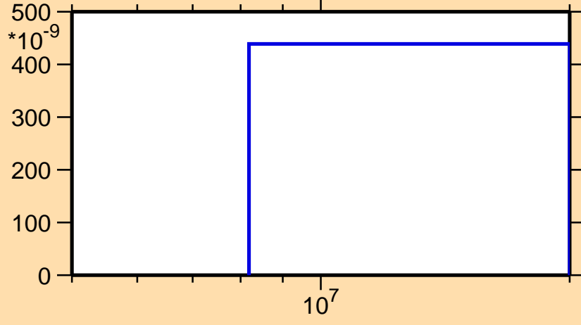
\sigma vs. E for ^{168}\text{Tm}(n,2n\alpha)
