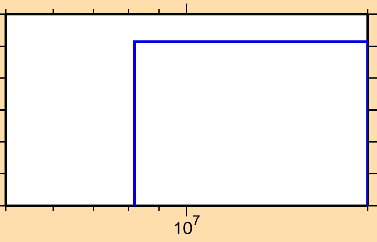
\sigma vs. E for ^{168}\text{Tm} (mt 45)
