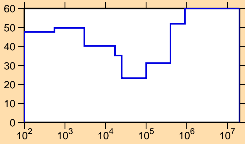
\Delta\sigma/\sigma vs. E for ^{168}\text{Tm}(n,\gamma)
