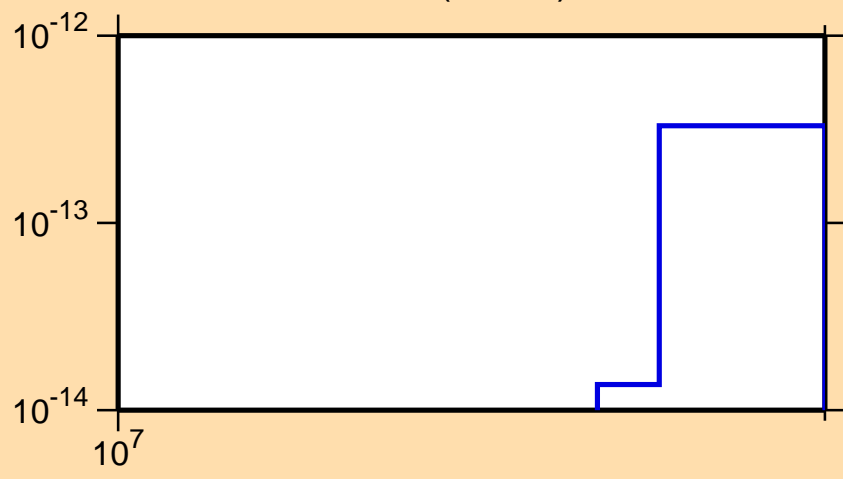
\sigma vs. E for ^{169}\text{Tm} (mt 45)
