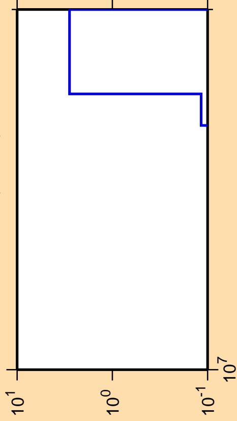
\Delta\sigma/\sigma vs. E for ^{169}\text{Tm} (mt 45)
