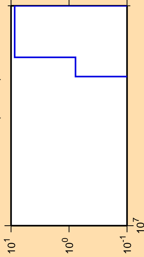
\Delta\sigma/\sigma vs. E for ^{169}\text{Tm}(\text{mt117})
