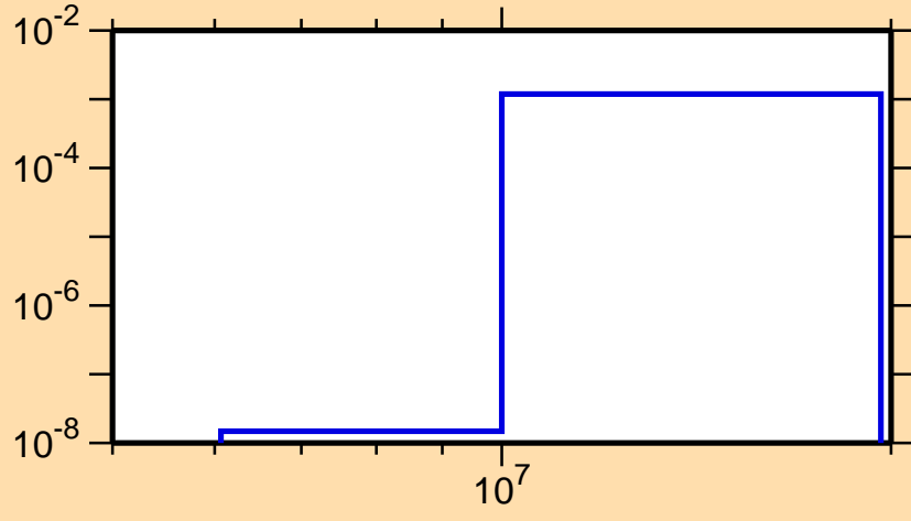
\sigma vs. E for ^{169}\text{Tm}(n,np)
