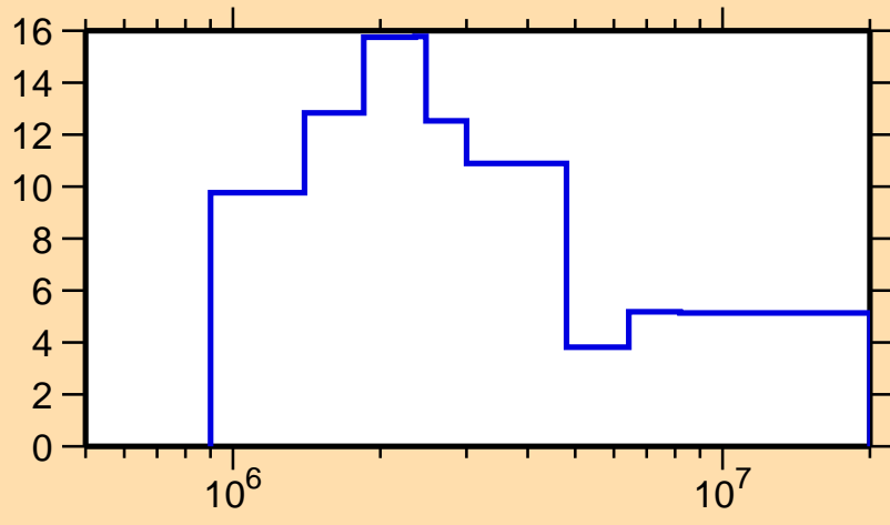
\Delta\sigma/\sigma vs. E for ^{169}\text{Tm}(n,el.)
