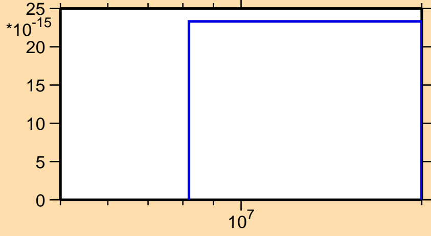
\sigma vs. E for ^{169}\text{Tm}(\text{mt117})
