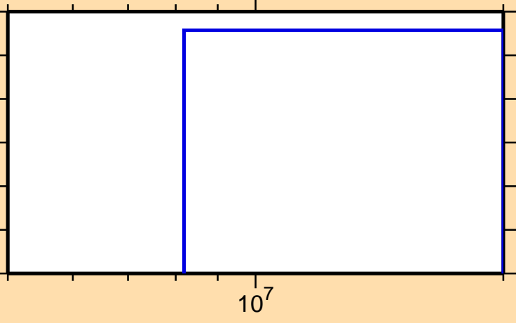
\sigma vs. E for ^{169}\text{Tm}(n,2np)
