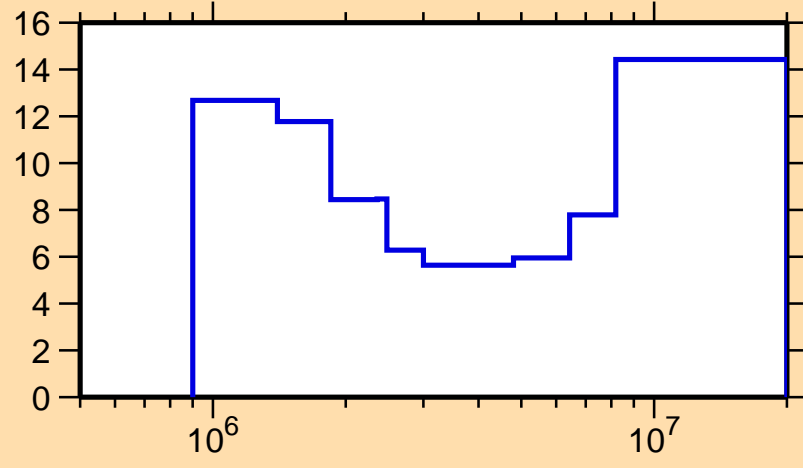
\Delta\sigma/\sigma vs. E for ^{169}\text{Tm}(n,ncont.)
