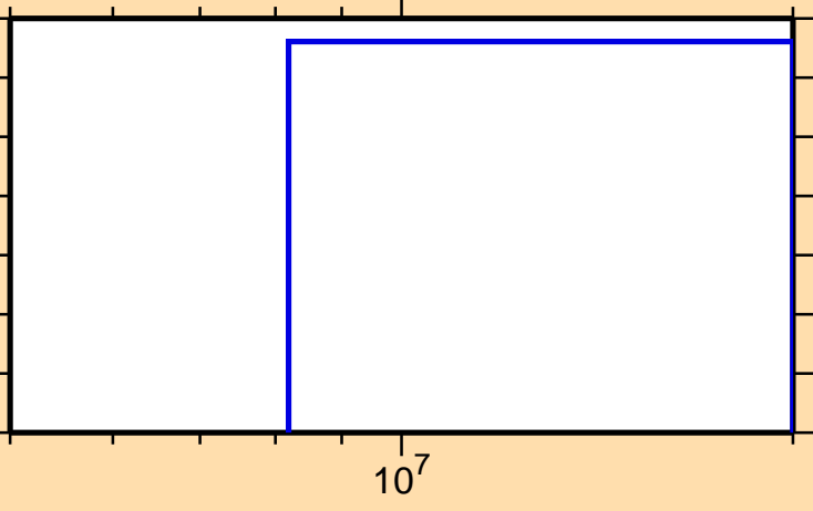
\sigma vs. E for ^{169}\text{Tm} (mt 45)
