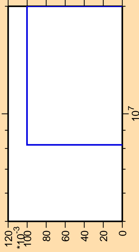
\Delta\sigma/\sigma vs. E for ^{169}\text{Tm}(\text{mt117})
