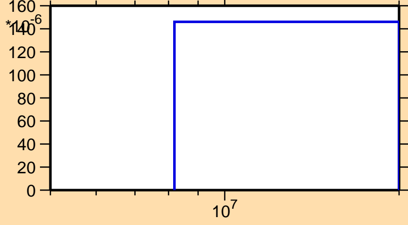
\sigma vs. E for ^{169}\text{Tm}(n,t)
