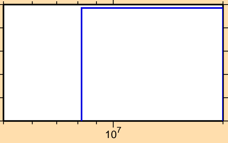
\sigma vs. E for ^{169}\text{Tm}(n,nd)
