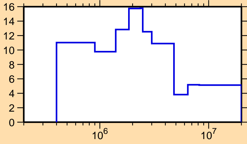
\Delta\sigma/\sigma vs. E for ^{169}\text{Tm}(n, el.)
