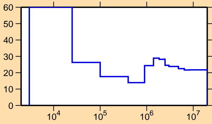
\Delta\sigma/\sigma vs. E for ^{169}\text{Tm}(n,n_1)
