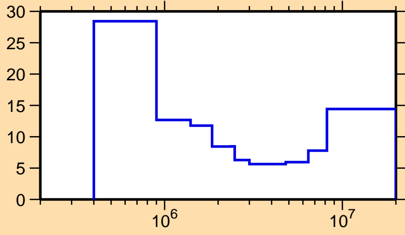
\Delta\sigma/\sigma vs. E for ^{169}\text{Tm}(n,n\text{cont.})
