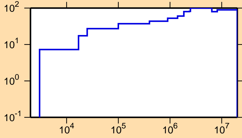
\Delta\sigma/\sigma vs. E for ^{169}\text{Tm}(n,\gamma)
