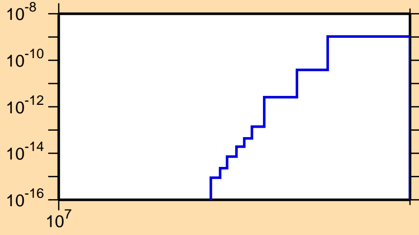
\sigma vs. E for ^{170}\text{Tm}(n,\text{He}3)
