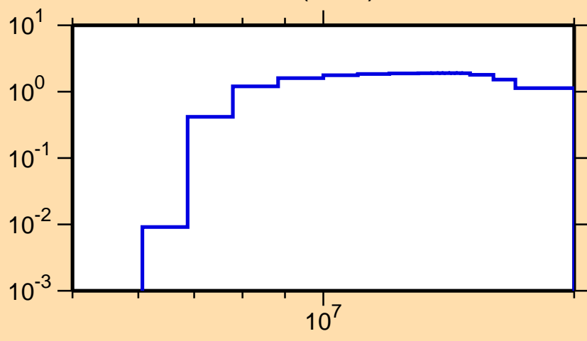
\sigma vs. E for ^{170}\text{Tm}(n,2n)
