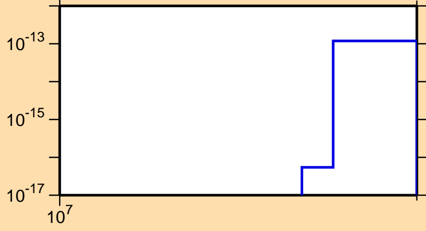
\sigma vs. E for ^{170}\text{Tm}(n,3n\alpha)
