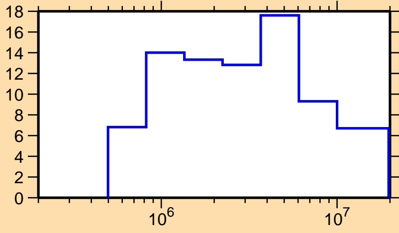
\Delta\sigma/\sigma vs. E for ^{170}\text{Tm}(n,el.)
