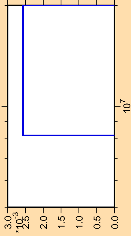
\Delta\sigma/\sigma vs. E for ^{170}\text{Tm}(n,3n\alpha)
