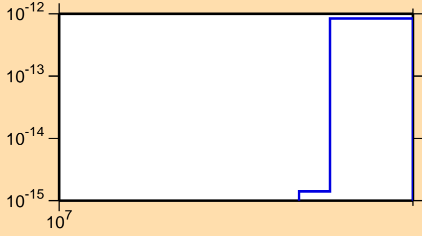
\sigma vs. E for ^{171}\text{Tm}(n,3n\alpha)
