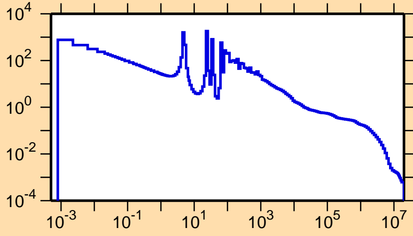
\sigma vs. E for ^{171}\text{Tm}(n,\gamma)
