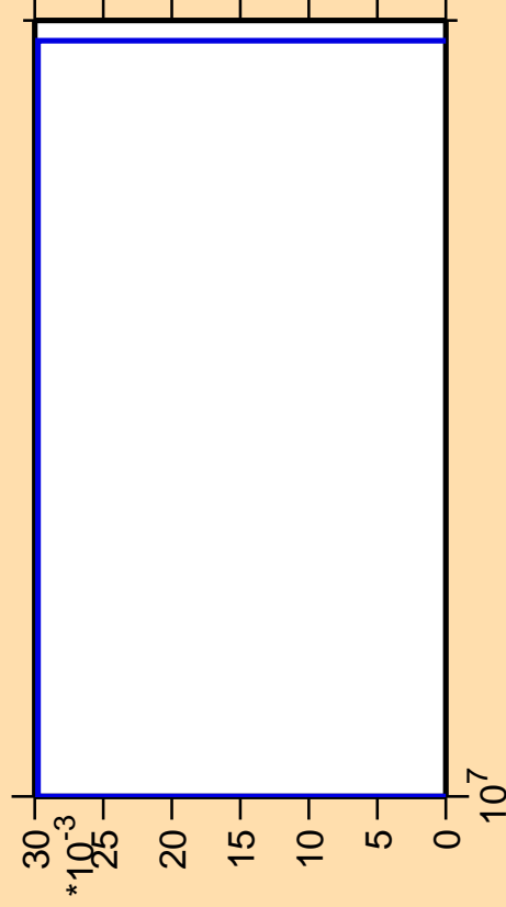
\Delta\sigma/\sigma vs. E for ^{171}\text{Tm}(n,3n\alpha)
