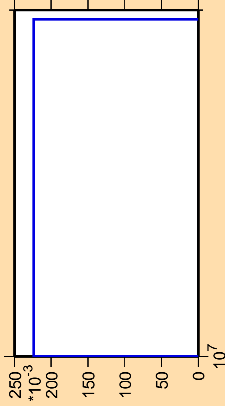
\Delta\sigma/\sigma vs. E for ^{171}\text{Tm}(n,p\alpha)
