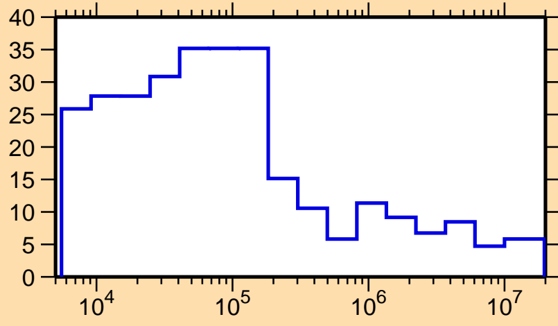
\Delta\sigma/\sigma vs. E for ^{171}\text{Tm}(n,\text{el.})
