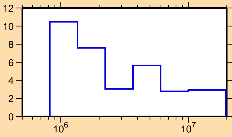
\Delta\sigma/\sigma vs. E for ^{171}\text{Tm}(n, tot.)
