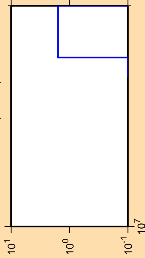
\Delta\sigma/\sigma vs. E for ^{172}\text{Tm}(n,3n\alpha)
