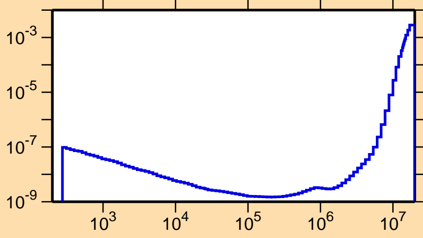
\sigma vs. E for ^{172}\text{Tm}(n,\alpha)
