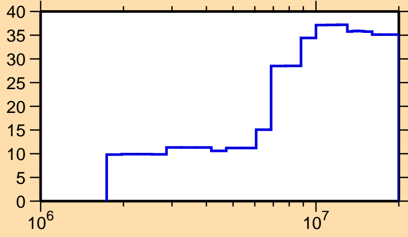
\Delta\sigma/\sigma vs. E for ^{172}\text{Tm}(n,ncont.)
