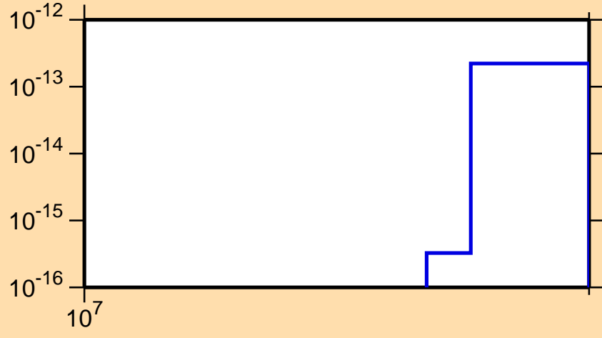
\sigma vs. E for ^{172}\text{Tm}(n,3n\alpha)
