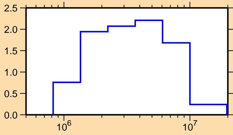
\sigma vs. E for ^{172}\text{Tm}(n,n\text{cont.})
