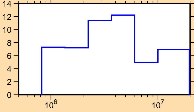
\Delta\sigma/\sigma vs. E for ^{172}\text{Tm}(n,el.)
