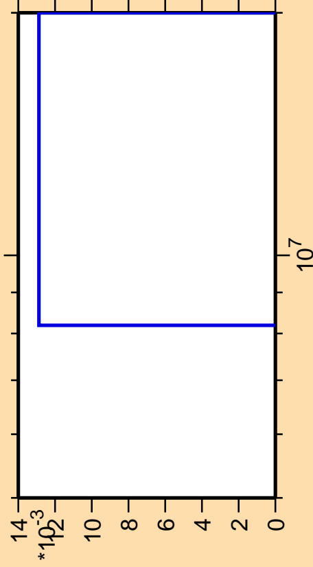
\Delta\sigma/\sigma vs. E for ^{172}\text{Tm}(n,3n\alpha)
