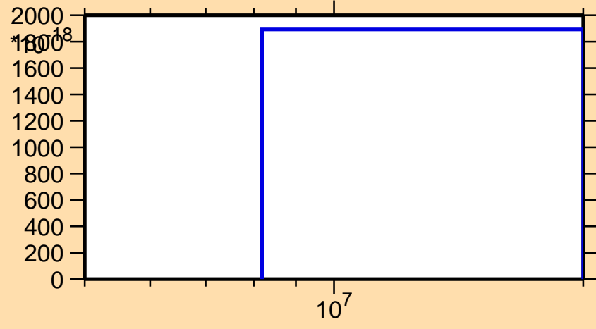
\sigma vs. E for ^{172}\text{Tm}(n,3n\alpha)
