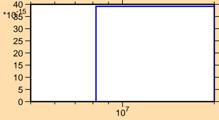
\sigma vs. E for ^{172}\text{Tm}(n,p\alpha)
