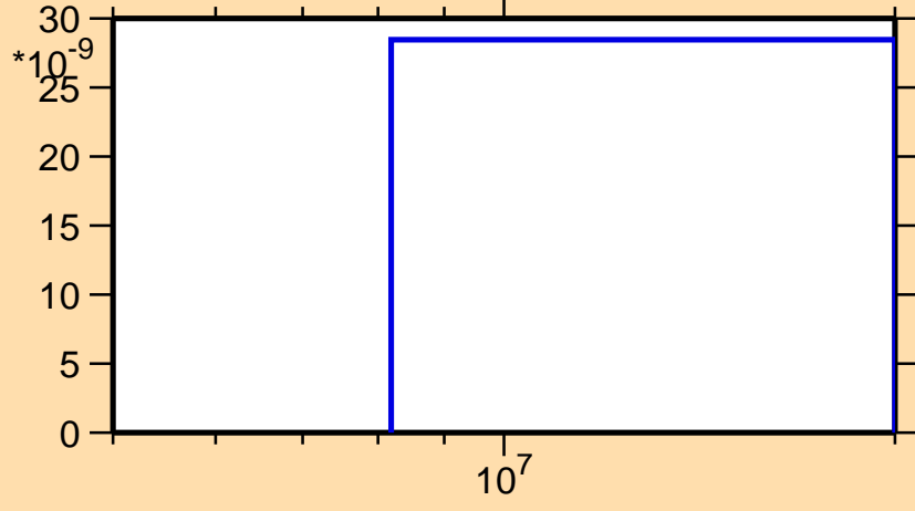
\sigma vs. E for ^{172}\text{Tm}(n,2n\alpha)
