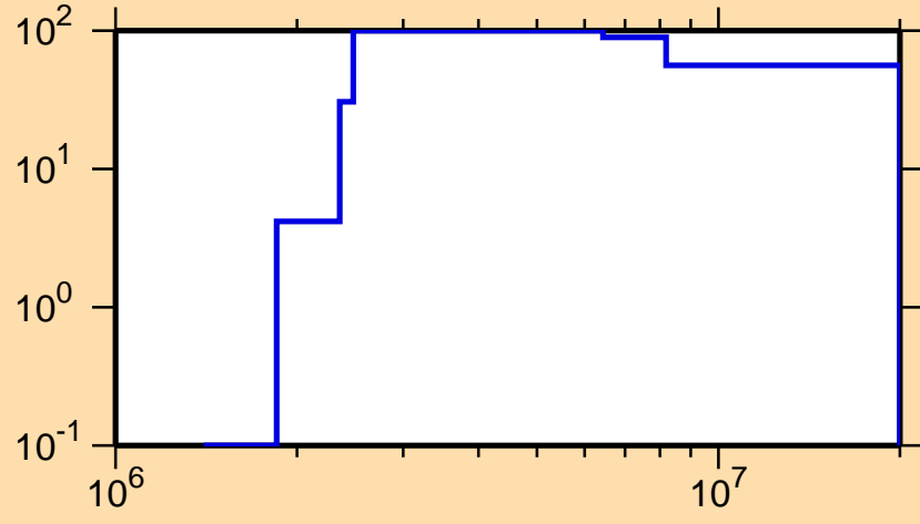
\Delta\sigma/\sigma vs. E for ^{172}\text{Tm}(n,p)
