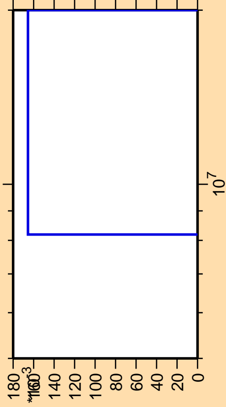
\Delta\sigma/\sigma vs. E for ^{172}\text{Tm}(n,p\alpha)
