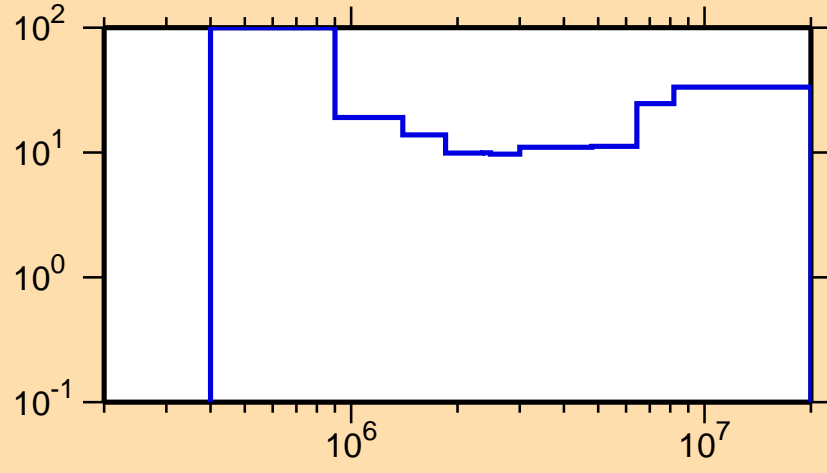
\Delta\sigma/\sigma vs. E for ^{172}\text{Tm}(n,n\text{cont.})
