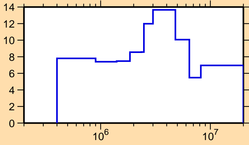
\Delta\sigma/\sigma vs. E for ^{172}\text{Tm}(n, el.)
