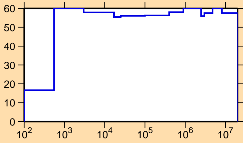
\Delta\sigma/\sigma vs. E for ^{172}\text{Tm}(n,\gamma)
