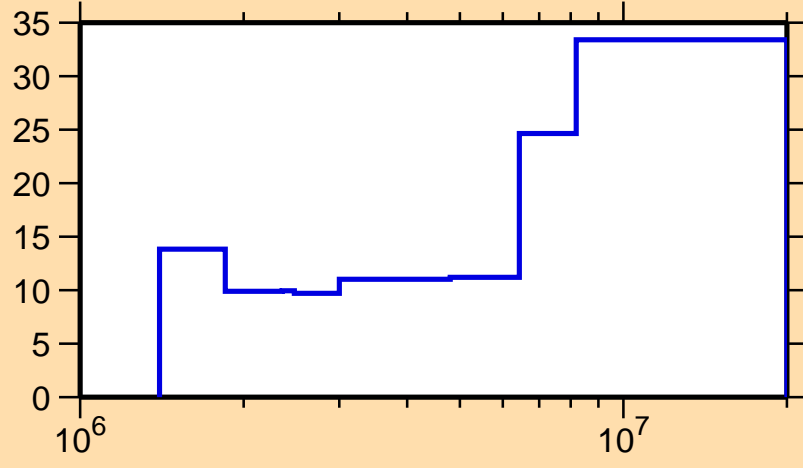
\Delta\sigma/\sigma vs. E for ^{172}\text{Tm}(n,ncont.)
