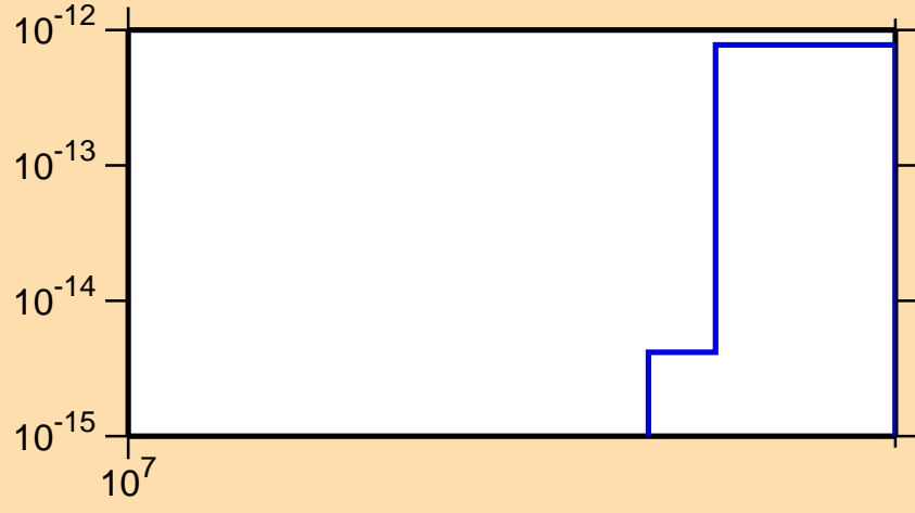
\sigma vs. E for ^{173}\text{Tm}(n,3n\alpha)
