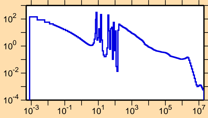
\sigma vs. E for ^{173}\text{Tm}(n,\gamma)
