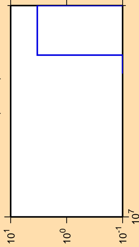
\Delta\sigma/\sigma vs. E for ^{173}\text{Tm}(n,3n\alpha)
