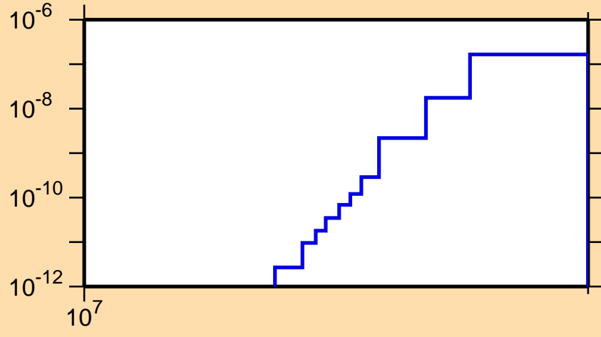
\sigma vs. E for ^{173}\text{Tm}(n,2n\alpha)
