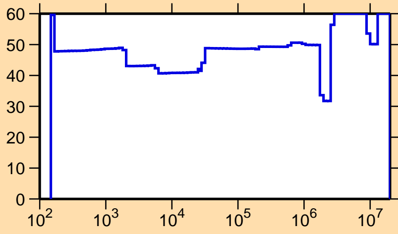
\Delta\sigma/\sigma vs. E for ^{173}\text{Tm}(n,\gamma)
