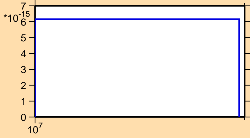
\sigma vs. E for ^{173}\text{Tm}(n,3n\alpha)
