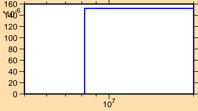
\sigma vs. E for ^{173}\text{Tm}(n,np)
