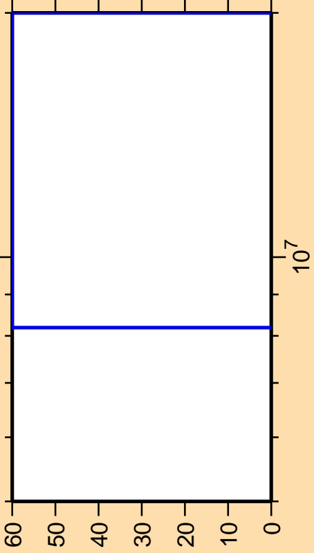
\Delta\sigma/\sigma vs. E for ^{173}\text{Tm}(n,nt)
