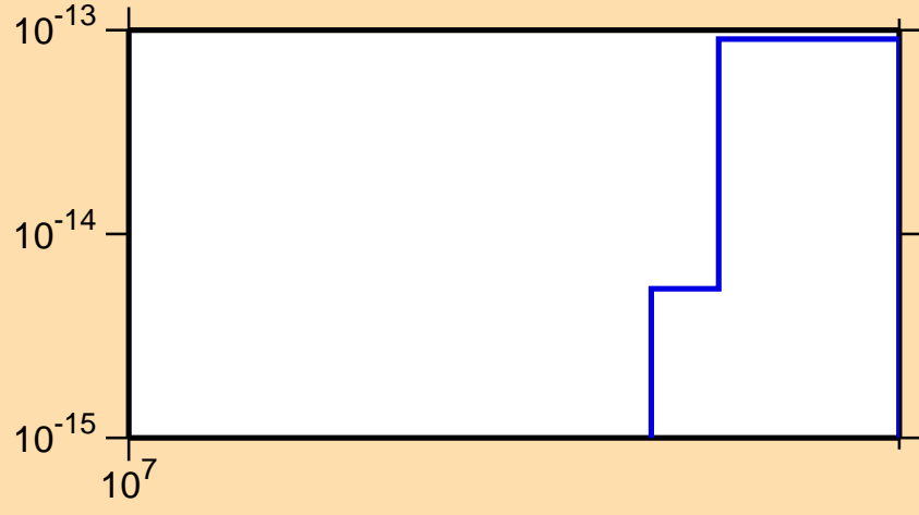
\sigma vs. E for ^{174}\text{Tm}(n,3n\alpha)
