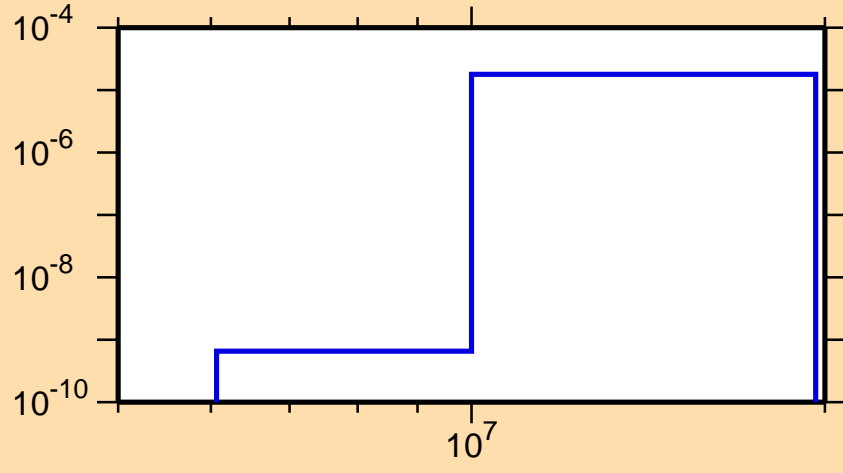
\sigma vs. E for ^{174}\text{Tm}(n,\alpha)
