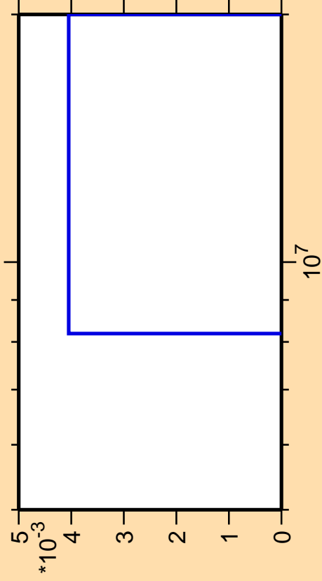
\Delta\sigma/\sigma vs. E for ^{174}\text{Tm}(n,3n\alpha)
