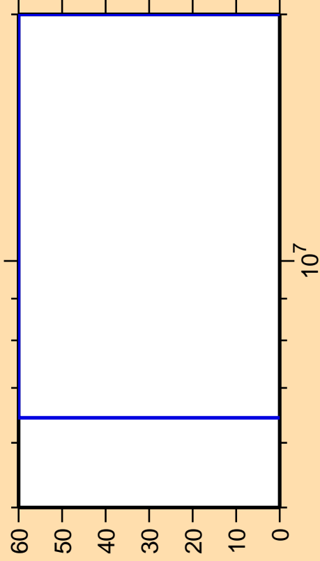
\Delta\sigma/\sigma vs. E for ^{174}\text{Tm}(n,n\alpha)
