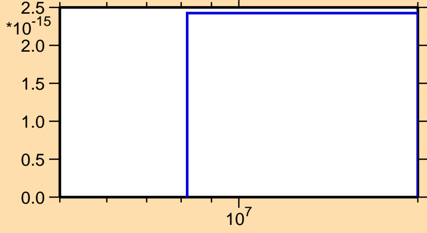
\sigma vs. E for ^{174}\text{Tm}(n,3n\alpha)
