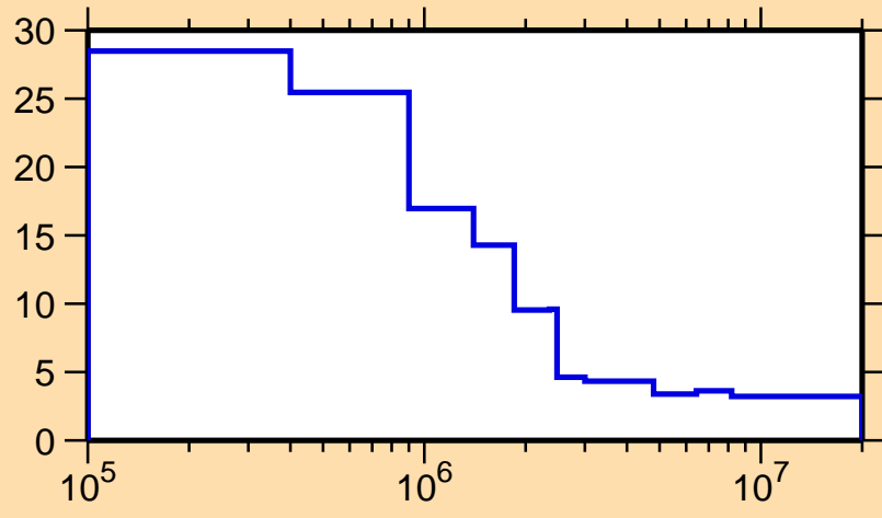
\Delta\sigma/\sigma vs. E for ^{174}\text{Tm}(n,\text{nonel.})
