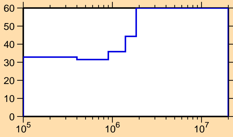
\Delta\sigma/\sigma vs. E for ^{174}\text{Tm}(n,n_1)
