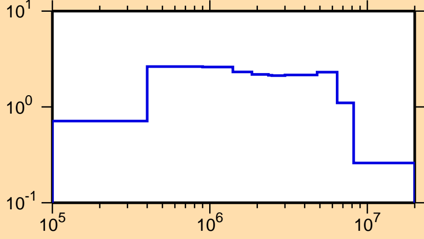
\sigma vs. E for ^{174}\text{Tm}(n,n\text{cont.})
