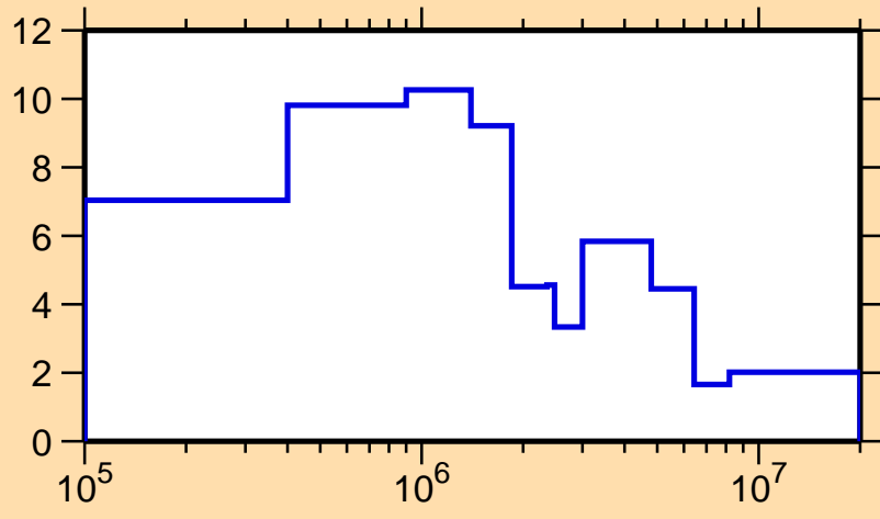
\Delta\sigma/\sigma vs. E for ^{174}\text{Tm}(n,\text{tot.})
