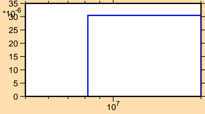
\sigma vs. E for ^{174}\text{Tm}(n,t)
