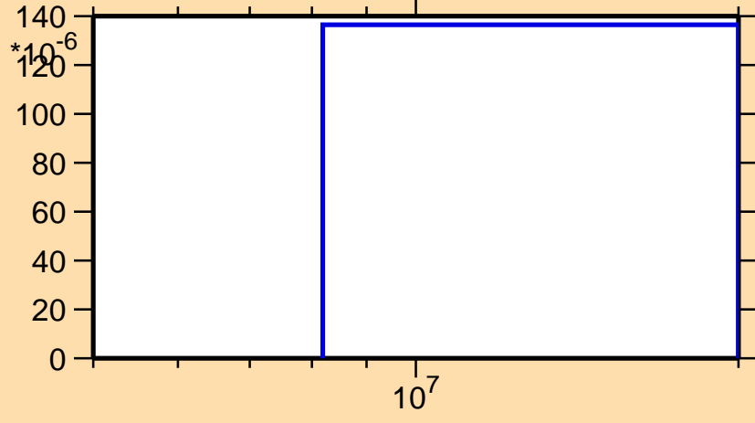
\sigma vs. E for ^{174}\text{Tm}(n,np)
