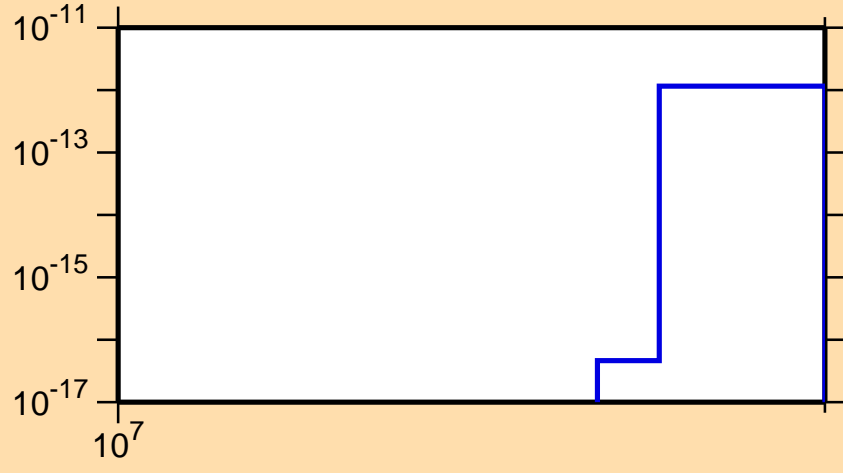
\sigma vs. E for ^{175}\text{Tm}(n,3n\alpha)
