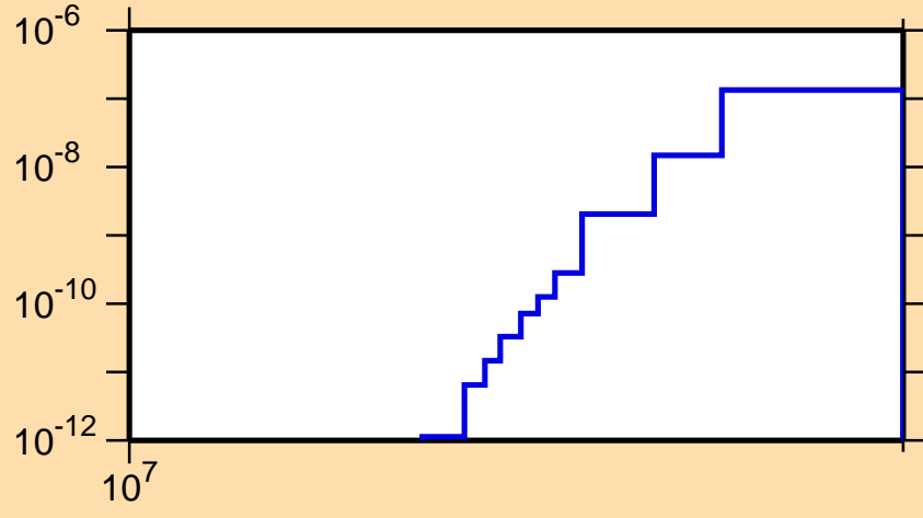
\sigma vs. E for ^{175}\text{Tm}(n,2n\alpha)
