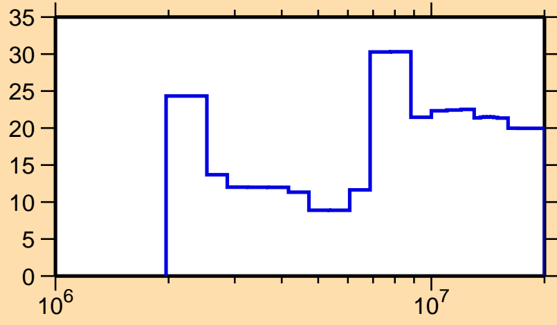
\Delta\sigma/\sigma vs. E for ^{175}\text{Tm}(n,n\text{cont.})
