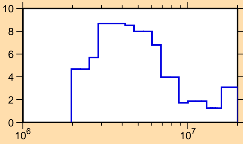
\Delta\sigma/\sigma vs. E for ^{175}\text{Tm}(n,\text{tot.})
