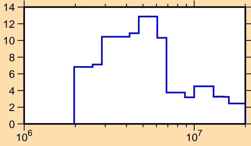
\Delta\sigma/\sigma vs. E for ^{175}\text{Tm}(n,el.)
