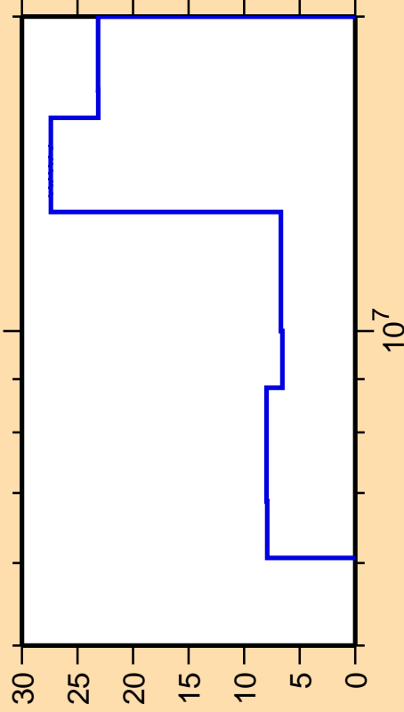
\Delta\sigma/\sigma vs. E for ^{175}\text{Tm}(n,2n)
