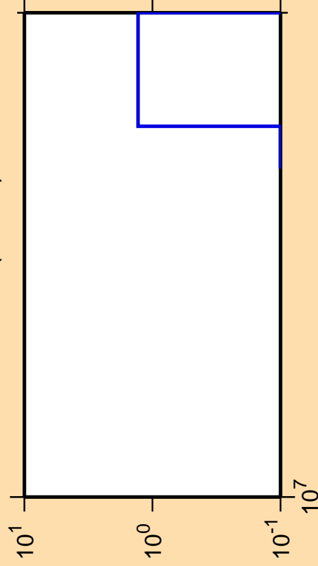
\Delta\sigma/\sigma vs. E for ^{175}\text{Tm}(n,3n\alpha)
