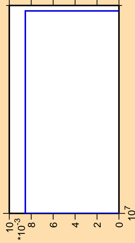
\Delta\sigma/\sigma vs. E for ^{175}\text{Tm}(n,3n\alpha)
