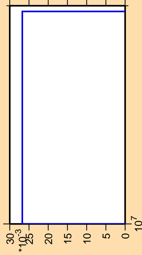
\Delta\sigma/\sigma vs. E for ^{176}\text{Tm}(n,3n\alpha)
