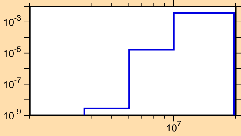
\sigma vs. E for ^{176}\text{Tm}(n,p)
