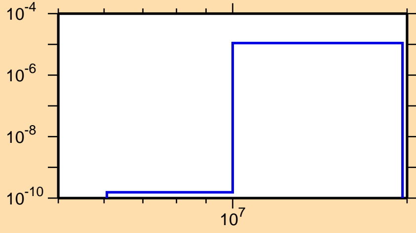
\sigma vs. E for ^{176}\text{Tm}(n,n\alpha)
