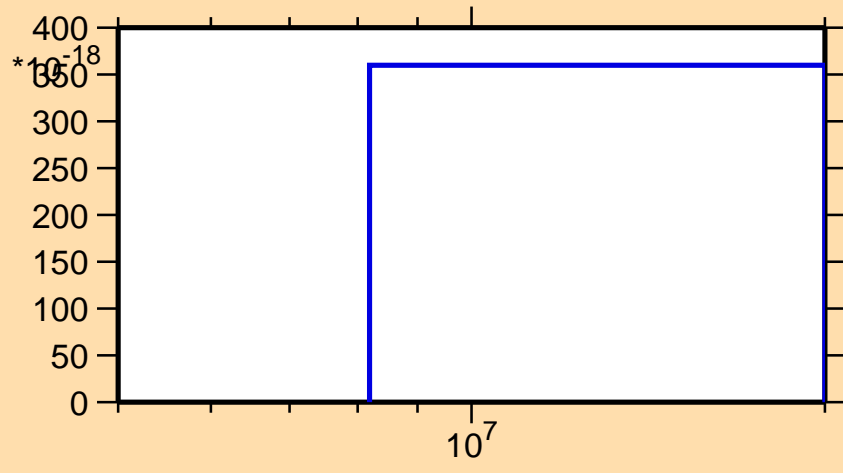
\sigma vs. E for ^{176}\text{Tm} (mt 11)
