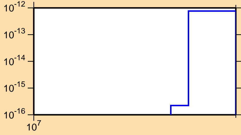
\sigma vs. E for ^{177}\text{Tm}(n,3n\alpha)
