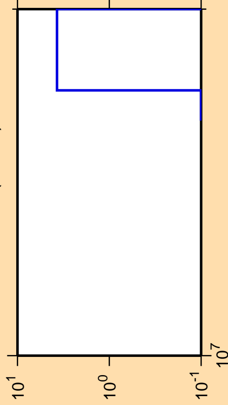
\Delta\sigma/\sigma vs. E for ^{177}\text{Tm}(n,3n\alpha)
