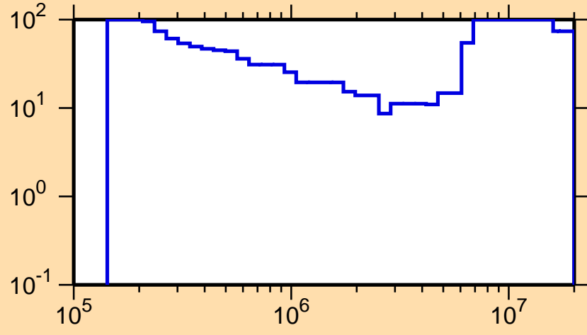
\Delta\sigma/\sigma vs. E for ^{177}\text{Tm}(n, inel.)
