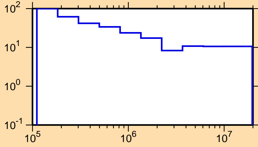
\Delta\sigma/\sigma vs. E for ^{177}\text{Tm}(n, nonel.)
