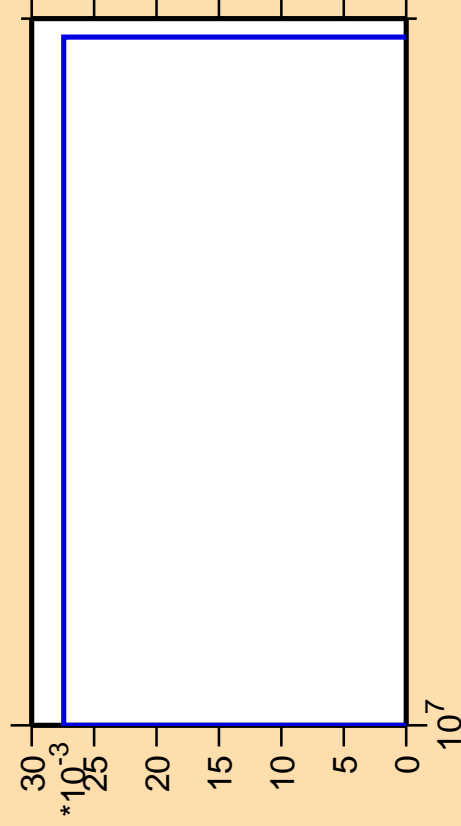
\Delta\sigma/\sigma vs. E for ^{177}\text{Tm}(n,3n\alpha)
