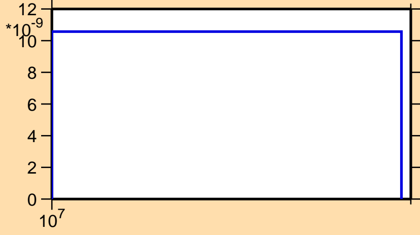
\sigma vs. E for ^{177}\text{Tm}(n,nd)
