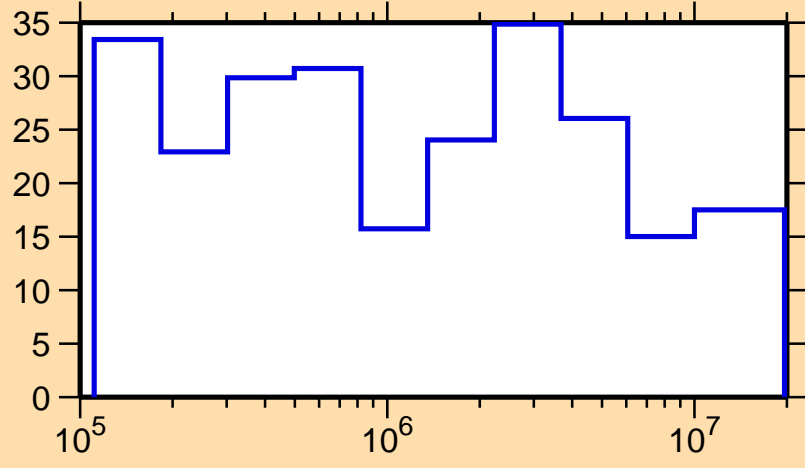
\Delta\sigma/\sigma vs. E for ^{177}\text{Tm}(n, el.)
