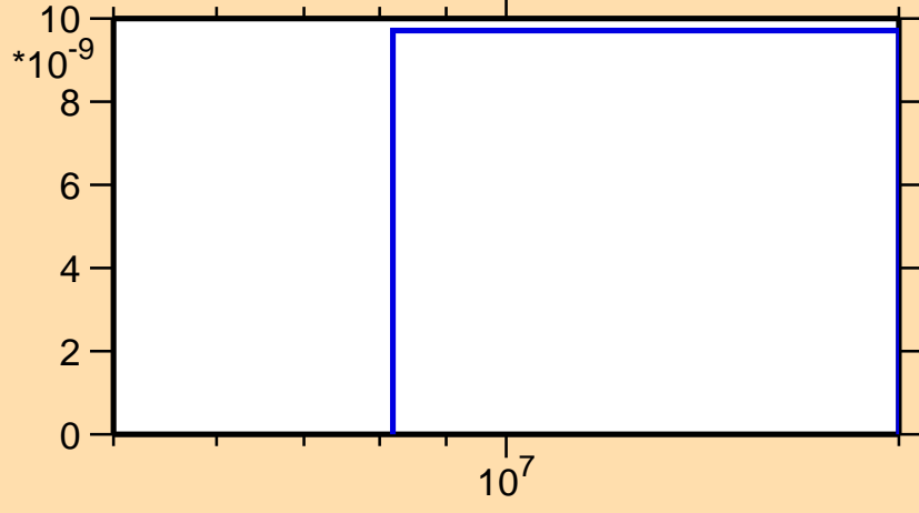
\sigma vs. E for ^{177}\text{Tm}(n,\text{nd})
