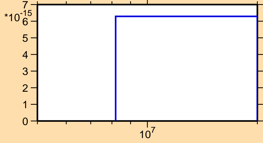
\sigma vs. E for ^{177}\text{Tm}(n,3n\alpha)
