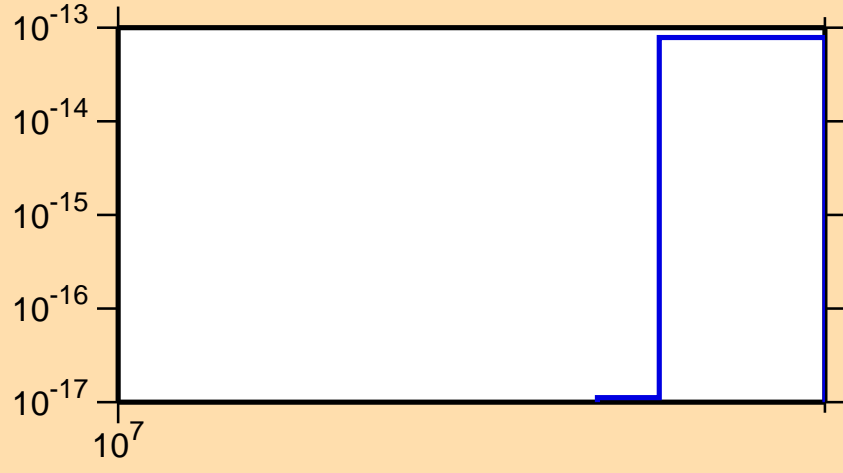
\sigma vs. E for ^{178}\text{Tm} (mt 11)
