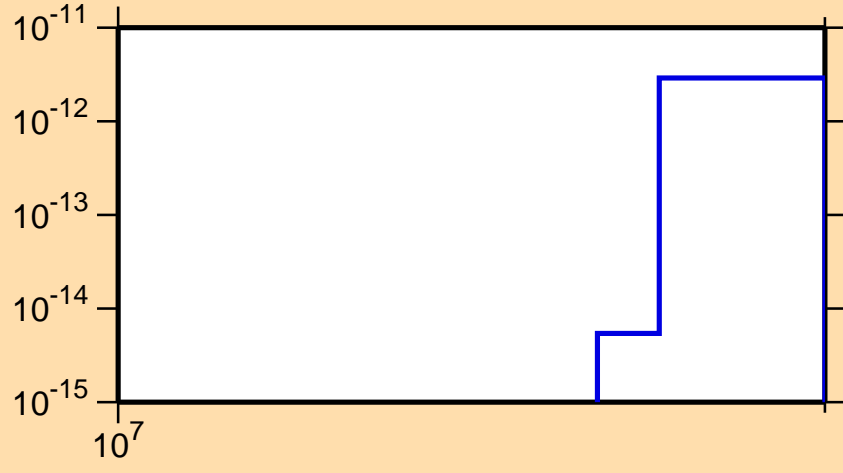
\sigma vs. E for ^{178}\text{Tm}(n,3n\alpha)
