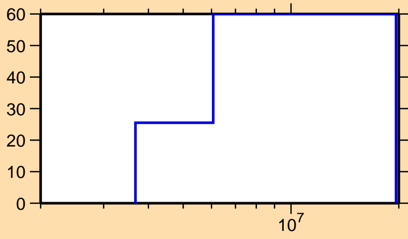
\Delta\sigma/\sigma vs. E for ^{178}\text{Tm}(n,p)
