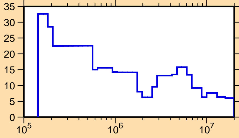
\Delta\sigma/\sigma vs. E for ^{179}\text{Tm}(n, el.)
