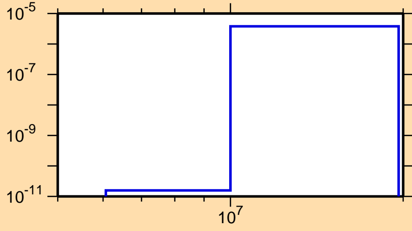
\sigma vs. E for ^{179}\text{Tm}(n,n\alpha)
